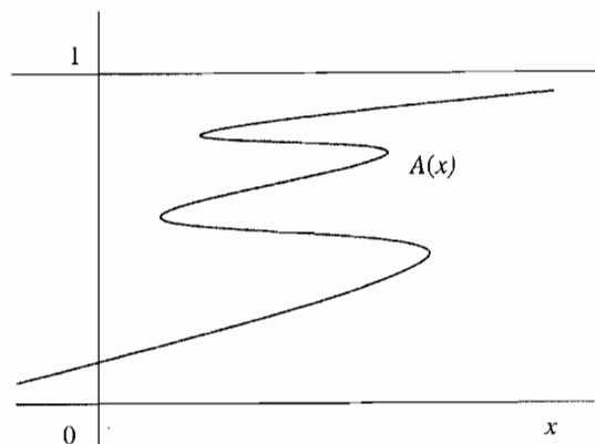
FIGURE 2. Complete information equilibria.
