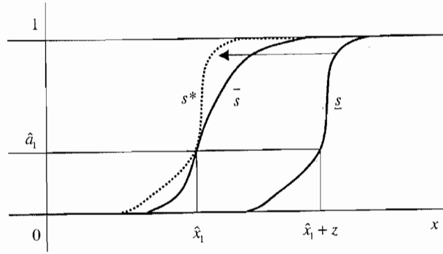
FIGURE 3 Translation argument.
