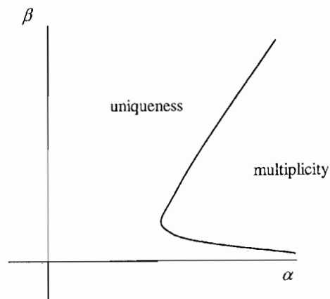
FIGURE 8 Private values uniqueness region.
