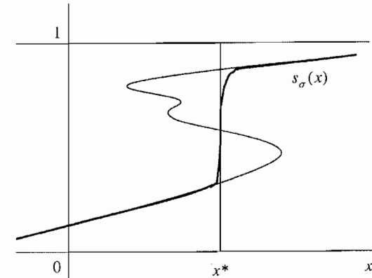
FIGURE 6 Unique equilibrium for small \sigma .
