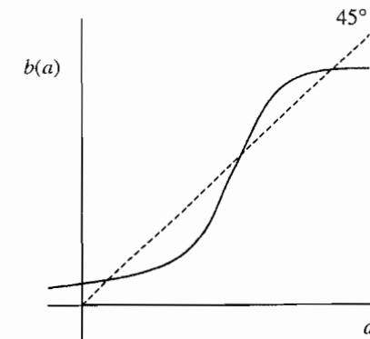
FIGURE 1 Best response function.
