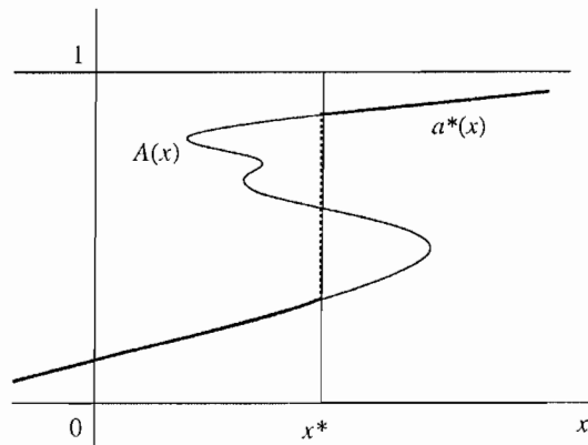
FIGURE 5 Selected equilibrium in limit.
