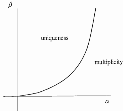
FIGURE 7 Common values uniqueness region.
