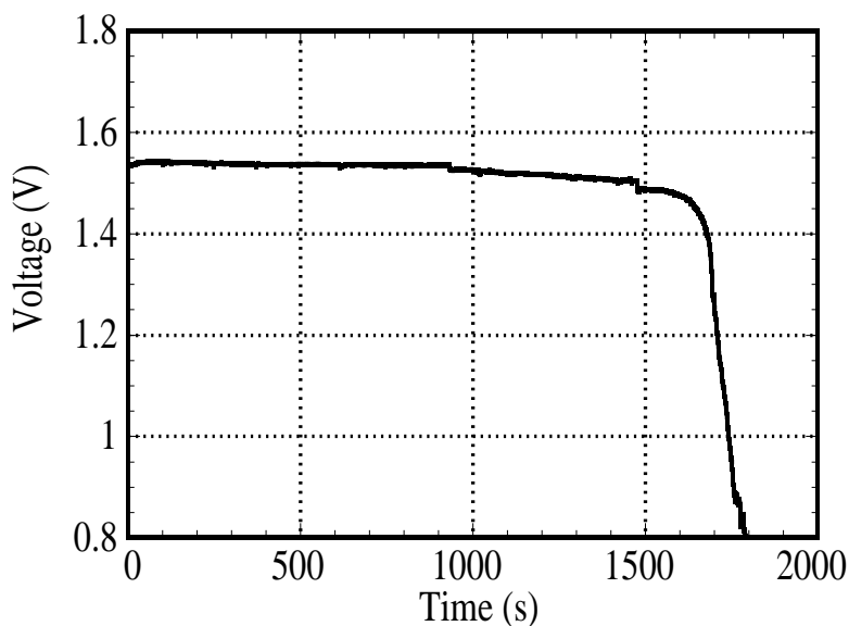
Figure 4. Discharge behavior of alkaline microbattery at 10 \mu\text{A} .
