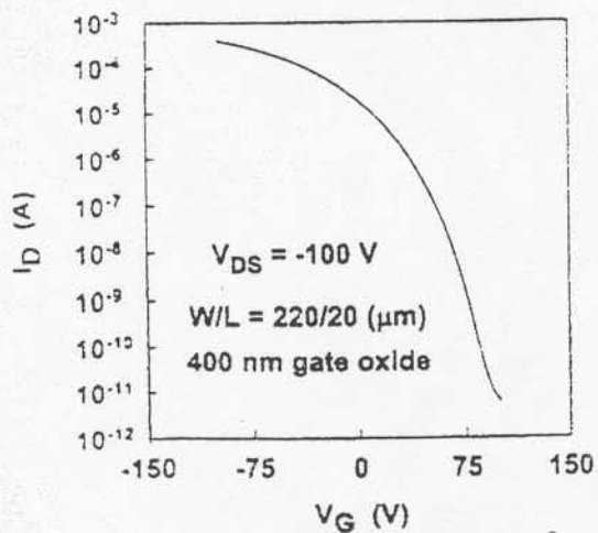
Pentacene TFT with I_{\text{on}}/I_{\text{off}} > 10^8
