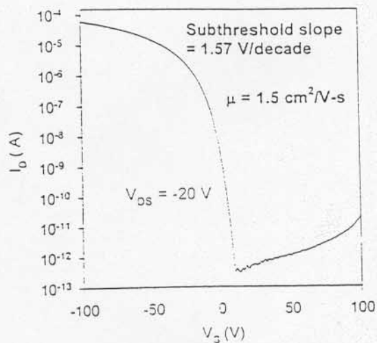
\text{Log}_{10}(I_D)\text{-}V_G characteristics for a lithographically-defined pentacene device.
