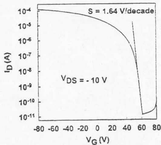
Pentacene/Octadecyltrichlorosilane TFT with 1.6 \text{ V/decade} subthreshold slope
