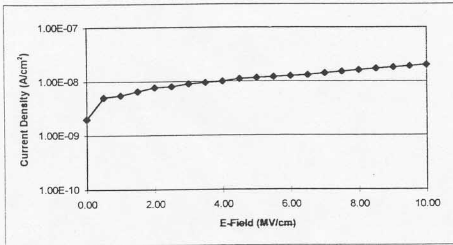
Figure 8 Low Temperature Device Quality ECR-PECVD Silicon Nitride
