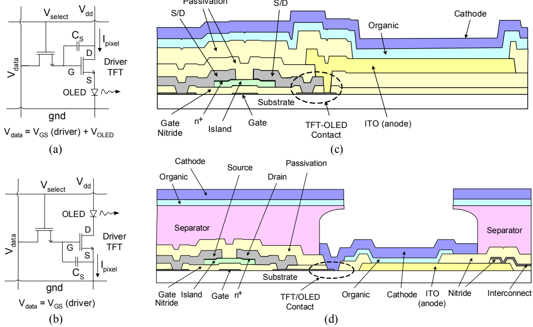
Fig. 1. Schematic circuit structure of a (a) normal and (b) a-Si AMOLED pixel. The cross section of the fabricated pixels is shown in (c) and (d) for the normal and inverted pixels, respectively.
