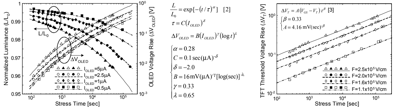
Fig. 2. Extraction of the individual TFT and OLED drifts. The OLED's are stressed at constant current densities and the TFT's at constant gate field ( F = V_{GS}/t_{SiNx} , nitride thickness = 300nm) for predicting the pixel reliability (Fig. 3).
