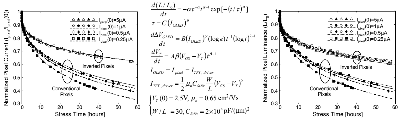
Fig. 3. Plots of the normalized pixel current drop and luminance decay for the normal and inverted pixels (symbols: data points, lines: predictions). The brightness decay is lower in the inverted pixels resulting in a higher pixel lifetime. The predictions are made by finding simultaneous solutions to the given set of differential equations (TFT/OLED decay rates). The fitting parameters are extracted by measuring TFT's and OLED's under constant DC stress (Fig. 2).
