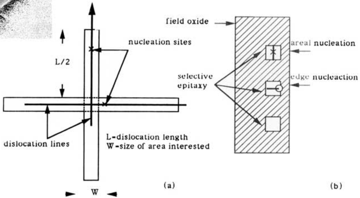
Fig.1 Schematic diagram illustrating concept of selective growth for enhanced metastability. In non-selective growth(a), the central W \times W area is susceptible to dislocations nucleated over a large cross area, which is decided by the dislocation length L . In the selective growth (b), the W \times W area is susceptible only to dislocations nucleated within that area, but edge nucleation must be considered.
