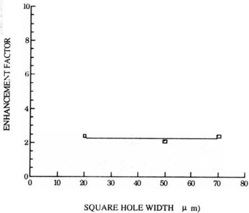
Fig. 5 Enhancement factor is a function of square width for \text{Si}_{.87}\text{Ge}_{.13} after 5 min. annealing at 900^\circ\text{C} . The constant EF indicates W is less than W_0 , i.e., edge nucleation is dominant.
