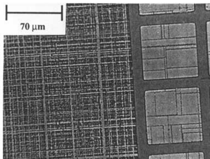
Fig. 4 The misfit dislocation network of \text{Si}_{0.87}\text{Ge}_{0.13} films of the thickness 200 nm annealed at 900 °C of various periods with {110} sidewall orientation to demonstrate the metastability enhancement of selective areas.
