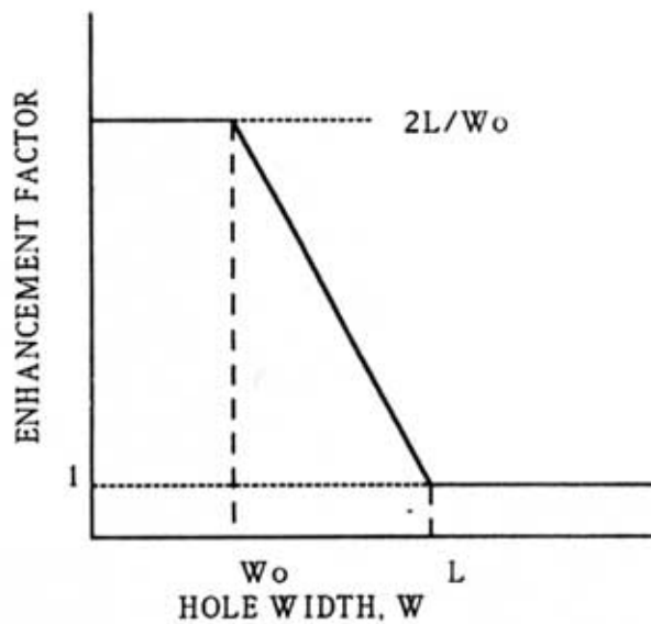
Fig.2 A schematic curve for Enhancement Factor as a function of size of selective area. For area size less than W_0 , the enhancement is limited by edge nucleation. For large area comparable with L , there is no enhancement at all. Between these two extremes, the enhancement factor is inversely proportional to the hole width.
