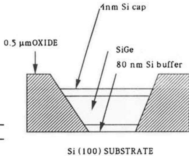
Fig. 3 The epitaxial structure of selective growth. The Si buffer and Si cap were grown at 900^\circ\text{C} and 700^\circ\text{C} , respectively. The SiGe was grown at 625^\circ\text{C}
