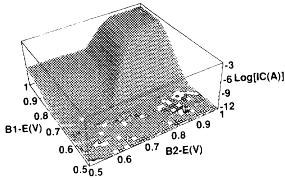
FIG. 6. Measured collector current of DBHBT No. 1077 at 77 K as a function of V_{B2} and V_{B1} .
