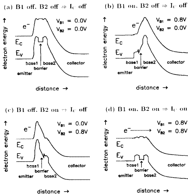
FIG. 2. Band diagrams showing modes of operation of DBHBT. Only if both base inputs are forward biased with respect to the emitter are electrons injected into the p -base region.
