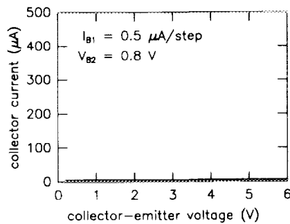
FIG. 7. Common-emitter characteristics (with input current into base 1) of DBHBT at 85 K for V_{B2} of (a) 1.0 V, and (b) 0.8 V showing control of the current gain I_C/I_{B1} by the voltage applied at the second base.
