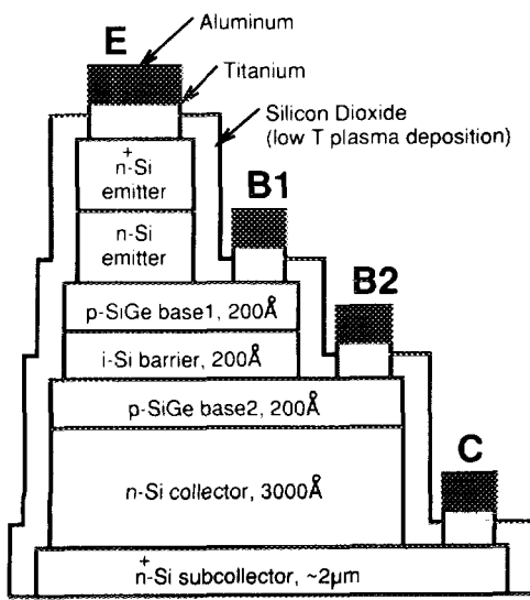
FIG. 3. Triple mesa device structure of DBHBT.
