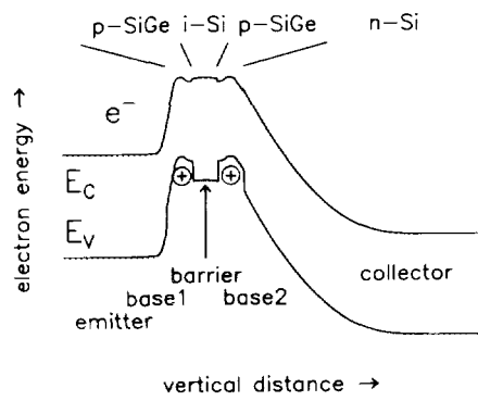
FIG. 1. Calculated band diagram of DBHBT, obtained by inserting an intrinsic silicon layer into the p -Si 1-x Ge x base of a flat-base HBT. Note that the conduction band in the base is still approximately flat because \Delta E_c \ll \Delta E_v at the Si/Si 1-x Ge x heterojunction.
