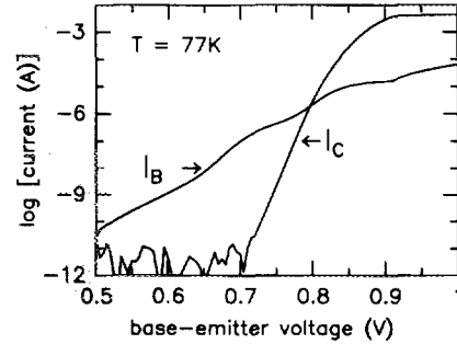
FIG. 4. Gummel plot of DBHBT No. 1077 at (a) room temperature and (b) 77 K with both bases externally shorted together and a base-collector reverse bias of 1 V.
