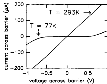
FIG. 5. Current-voltage characteristics of the p -Si 1-x Ge x / i -Si/ p -Si 1-x Ge x barrier of device No. 1077 at room temperature and at 77 K.
