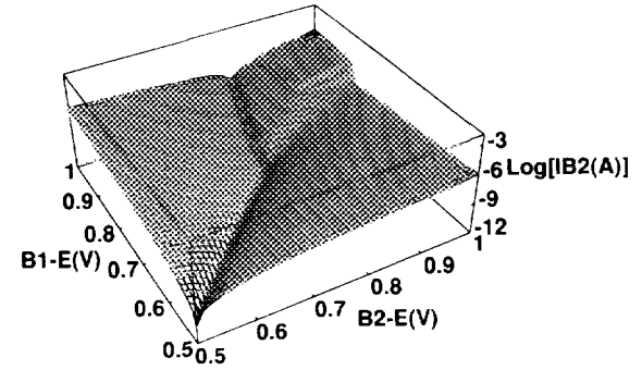
FIG. 8. Measured magnitude of the current into (a) base 1 and (b) base 2 vs input voltages of device No. 1077 at 77 K.
