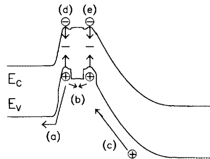
FIG. 9. Schematic band diagram showing the source of the two base currents I_{B1} and I_{B2} .
