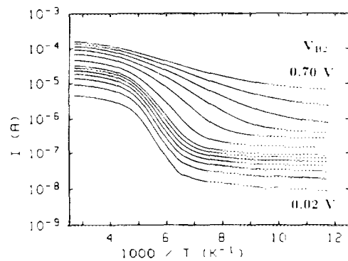
FIG. 11. Current across i -silicon barrier plotted logarithmically vs inverse temperature for various values of V_{B2} - V_{B1} (0.02, 0.04, ..., 0.14, 0.2, 0.3, ..., 0.7 V).
