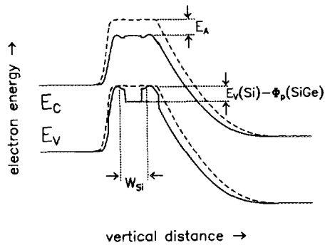
FIG. 10. Band diagram of DBHBT (solid lines) and Si homojunction transistor (dashed lines) showing the parameters determined from electrical measurements: barrier thickness W_{Si} ; effective band gap reduction E_A ; and barrier height for holes, E_V(Si) - \Phi_p(SiGe) .
