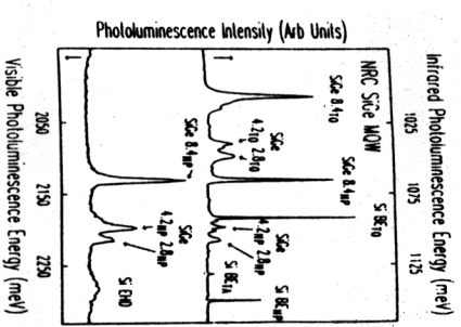
Figure 1. Comparison of the IR (top) and visible (bottom) spectra of a 3 well (2.8, 4.2, 8.4 nm, 14% Ge) MBE sample. The arrows point to the corresponding energy scale. The sample temperature was \approx 1.7 K. For the IR and visible spectra the excitation was \approx 50 mW/cm 2 at 514.5 nm and \approx 50 W/cm 2 at 740 nm respectively. Features labeled BE are bound exciton recombination from the Si substrate. Features labeled TO are TO phonon replicas of the corresponding no-phonon (NP) lines.
