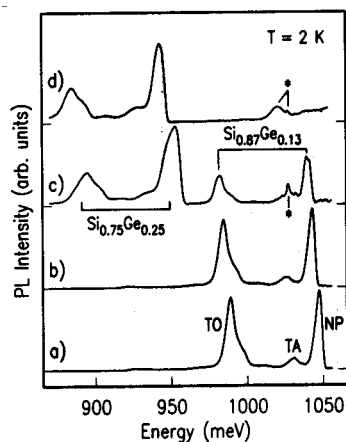
FIG. 2. Shift from outer-well to center-well luminescence with variation in Si barrier width. The outer-well PL, labeled \text{Si}_{0.87}\text{Ge}_{0.13} , is seen for (a) 15, (b) 12, and (c) 9 nm. In (d) 4 nm and (c) 9 nm, the barriers are thin enough to allow tunneling so that the center-well PL (labeled \text{Si}_{0.75}\text{Ge}_{0.25} ) is observed. In each case the NP peak is accompanied by TO and TA phonon replicas. The starred features originate from the Si substrate.
