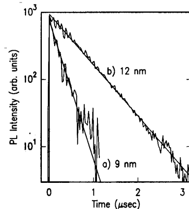
FIG. 4. Time decay of the outer-well PL ( \text{Si}_{0.87}\text{Ge}_{0.13} ) for (a) 9-nm Si barriers is faster than for (b) 12-nm Si barriers, consistent with the evidence of tunneling in the PL spectral features (Fig. 2). The solid lines show fits to the data which correspond to lifetimes of (a) 210 and (b) 575 ns. The PL intensities have been scaled to give equal values at t=0 . The PL rise times are less than 50 ns, indicating that the dynamics of the carrier migration from the substrate to the wells is much faster than the PL decay.
