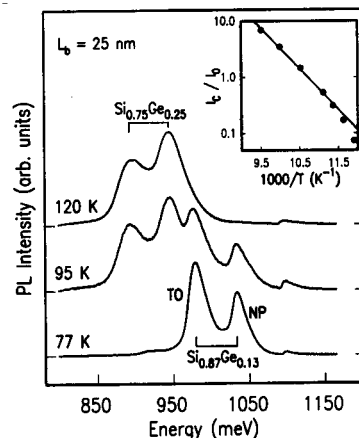
FIG. 3. Evolution of center-well ( \text{Si}_{0.75}\text{Ge}_{0.25} ) PL as the outer well ( \text{Si}_{0.87}\text{Ge}_{0.13} ) is depopulated by increasing the temperature from 77 to 95 K, then 120 K in a sample with no observed tunneling (25-nm Si barriers). The inset shows an Arrhenius plot of the center-well TO intensity ( I_c ) normalized by the outer-well NP peak ( I_o ). A fit to the data gives an activation energy of 145 meV, in agreement with the depth of the outer well as observed in the PL (132 meV).
