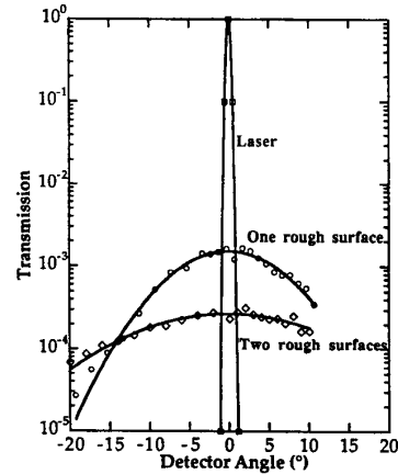
Fig. 4. Beam profiles of the original 1.3\text{-}\mu\text{m} probe beam after passing through one or two wafers (each with a single rough surface). The incident beam was at normal incidence.
