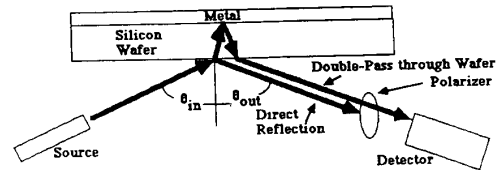
Fig. 1. Schematic diagram of the double-pass infrared transmission technique for the temperature measurement of metal-coated silicon wafers. Incident light at Brewster's angle was used to minimize the undesired direct reflection.
