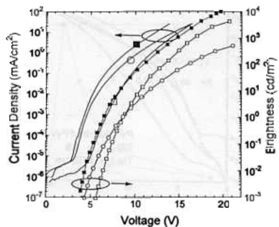
Fig. 20. Forward current-voltage-brightness characteristics of the blue (○), green (■), and orange (□) devices in Fig. 19.
