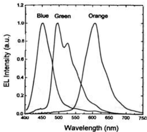
Fig. 19. EL spectra of blue, green, and orange devices, the compositions of which are ITO/PVK : PBD : C47(100 : 40 : 1 by wt.) /Mg : Ag/Ag, ITO/PVK : PBD : C6 (100 : 40 : 0.3 by wt.) /Mg : Ag/Ag and ITO/PVK : Alq : nile red (100 : 40 : 0.2 by wt.) /Mg : Ag/Ag, respectively.
