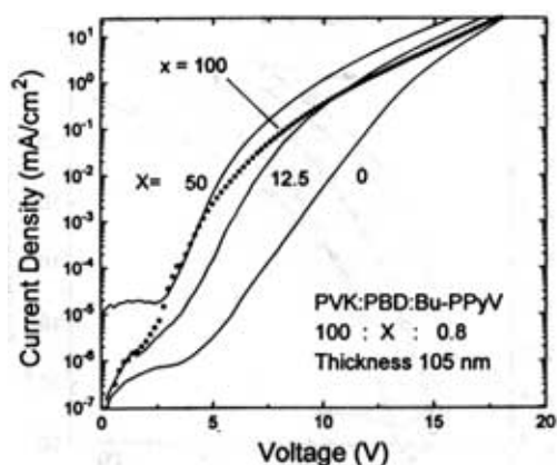
Fig. 16. Forward I - V characteristics of ITO/PVK : PBD : Bu-PPyV/Mg : Ag/Ag devices of different PBD contents.
