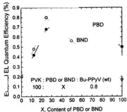
Fig. 15. External EL efficiency of ITO/PVK : PBD : Bu-PPyV/Mg : Ag/Ag devices and ITO/PVK : BND : Bu-PPyV/Mg : Ag/Ag devices versus content of PBD or BND.
