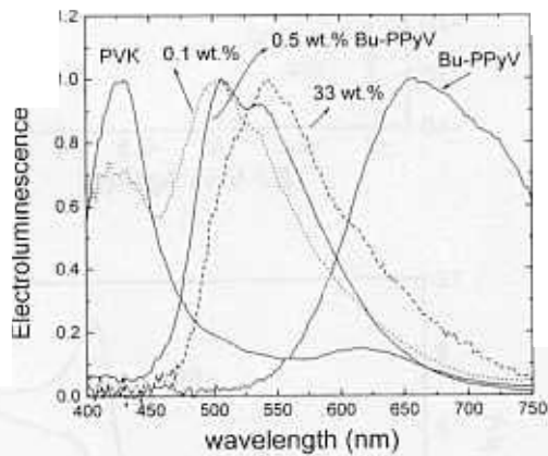
Fig. 11. Normalized EL spectra of PVK : Bu-PPyV devices of different Bu-PPyV contents.
