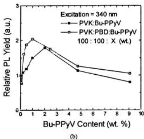
Fig. 6. (a) Photoluminescence spectra of Bu-PPyV : PVK blend thin films with different Bu-PPyV content. The excitation wavelength was 340 nm, with most absorption occurring in PVK as Bu-PPyV content is low. (b) Relative integrated photoluminescence efficiencies of PVK : Bu-PPyV and PVK : PBD : Bu-PPyV blend thin films versus Bu-PPyV content. The excitation wavelength was 340 nm. The strengths were normalized by the absorption at 340 nm in each film.
