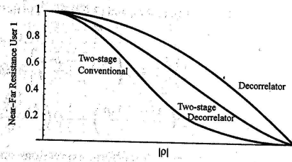
FIGURE 7.22. Near-far resistance of two-stage detector with conventional and decorrelating first stage for two synchronous users.
