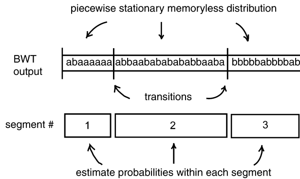
Fig. 2. Estimation of entropy after segmentation of the BWT output.
