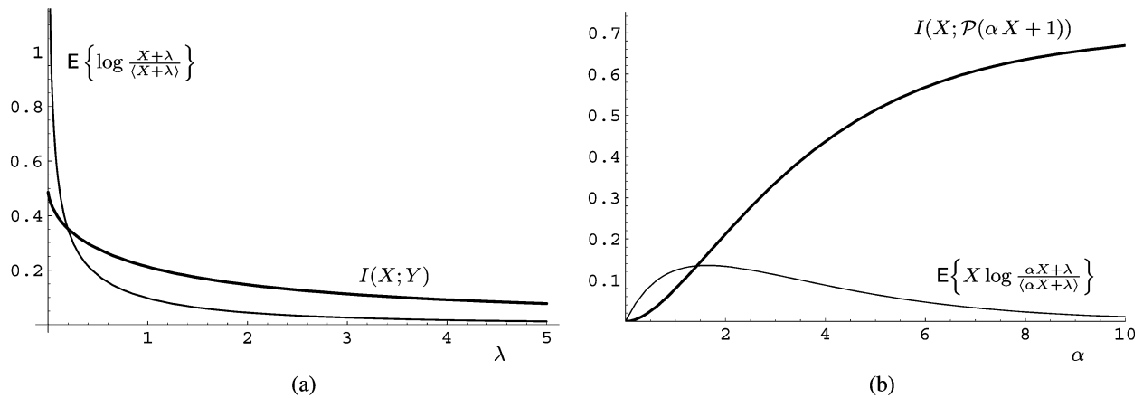
Fig. 3. Theorems 1 and 2 are verified for binary input. (a) The input is equally likely to be 0 and 2. The mutual information (in nats) and the expected error are plotted as a function of the dark current level. Unit scaling is assumed. (b) The mutual information (in nats) and the estimation error as functions of the scaling factor. The input X is binary and equally likely to be 0 and 1. Unit dark current is assumed ( \lambda = 1 ).
