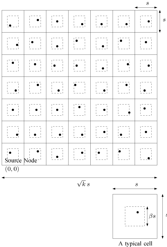
Fig. 4. Regular network.
