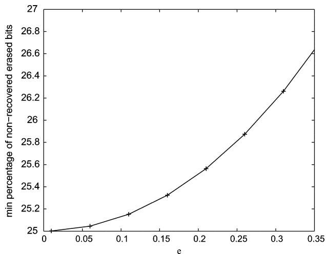
Fig. 8. \frac{100}{e} \mathbb{P}(\hat{X}_i \neq X_i) versus e , where \mathbb{P}(\hat{X}_i \neq X_i) is the probability of error of the optimal denoiser that knows the source distribution, and is computed using (20), for a BSMS with q = 0.25 passing through an erasure channel which erasure probability of e .
