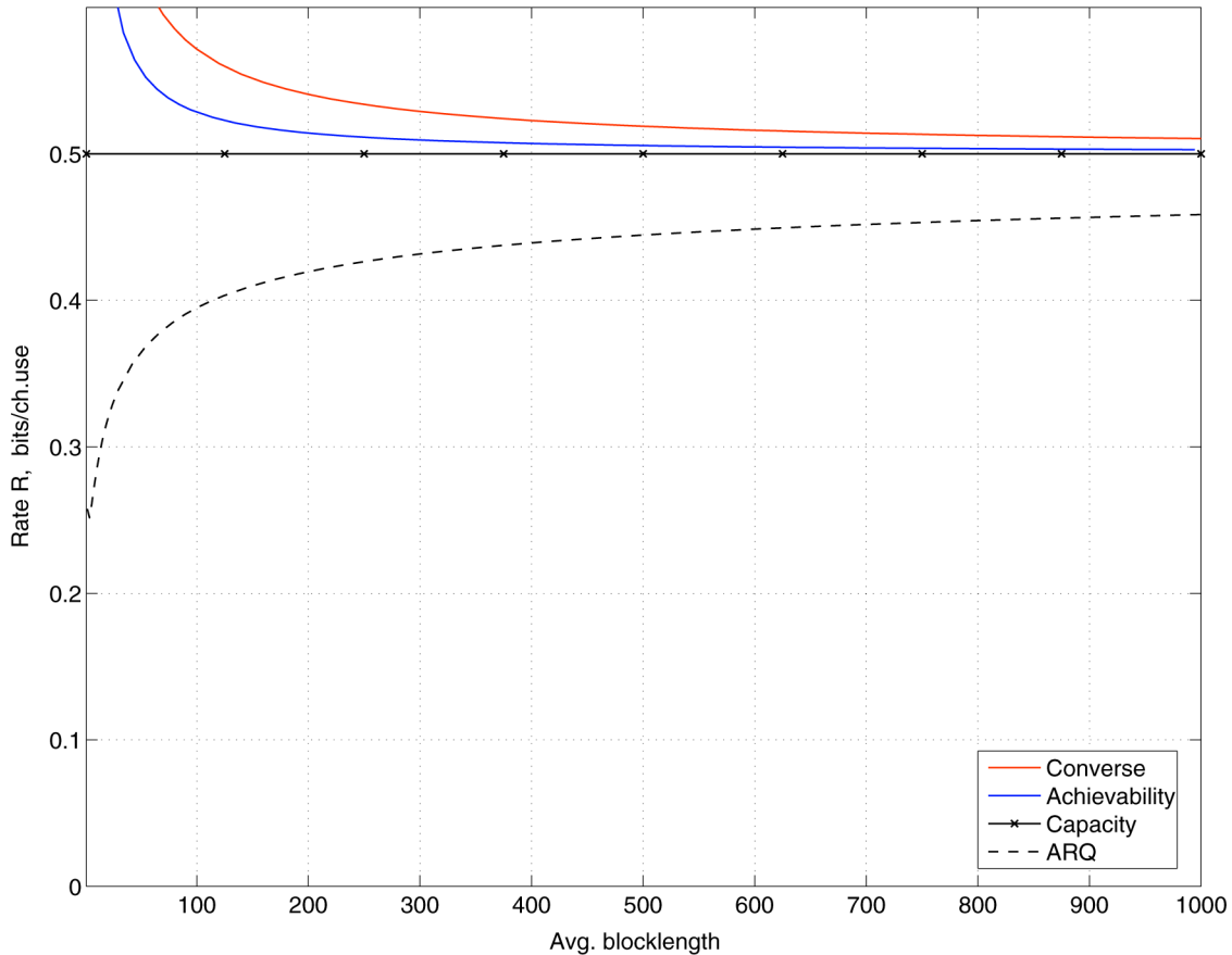
Fig. 4. Rate \frac{1}{\ell} \log M_i^*(\ell, 0) as a function of \ell for zero-error transmission over the BEC(0.5) with a termination symbol. The lower bound is Theorem 13; the upper-bound is (48).
