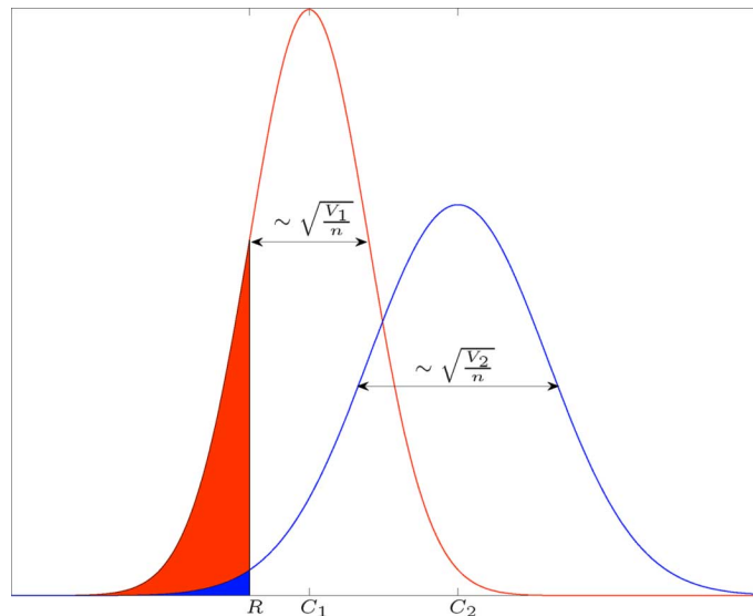
Fig. 4. Illustration to the Definition 2: R_{\text{na}}(n, \epsilon) is found as the unique point R at which the weighted sum of two shaded areas equals \epsilon .
