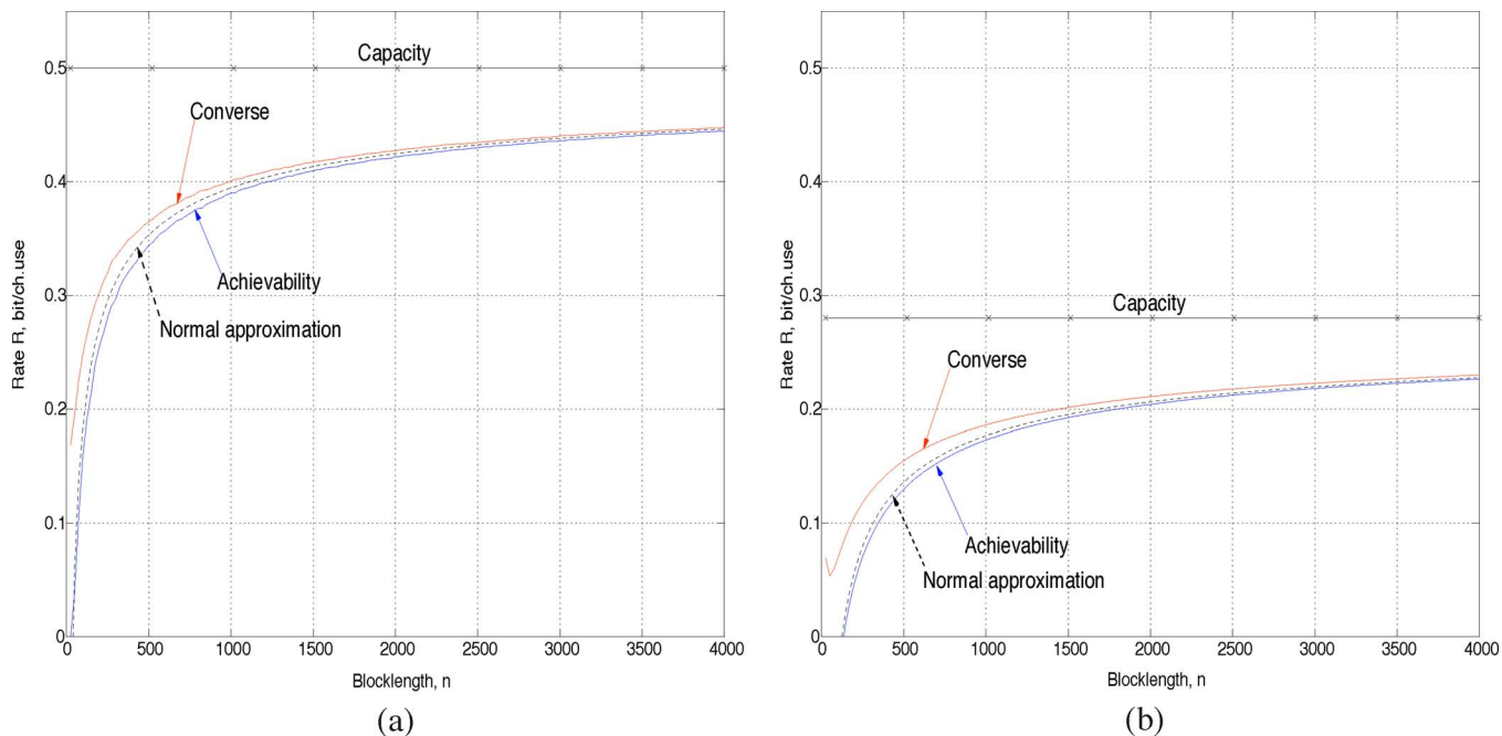
Fig. 1. Rate-blocklength tradeoff at block error rate \epsilon = 10^{-2} for the Gilbert-Elliott channel with parameters \delta_1 = 1/2 , \delta_2 = 0 and state transition probability \tau = 0.1 . (a) State S^n known at the receiver. (b) No state information.
