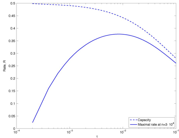
Fig. 3. Comparison of the capacity and the maximal achievable rate \frac{1}{n} \log M^*(n, \epsilon) at blocklength n = 3 \cdot 10^4 as a function of the state transition probability \tau for the Gilbert-Elliott channel with no state information at the receiver, \delta_1 = 1/2, \delta_2 = 0 ; probability of block error is \epsilon = 0.01 .
