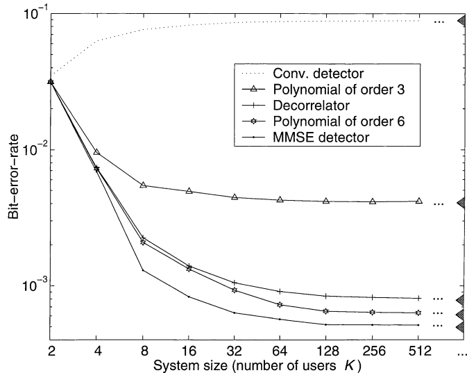
Fig. 4. BER versus the number of users (long sequences). The asymptotic estimates are marked by solid triangles on the right border of the plot.
