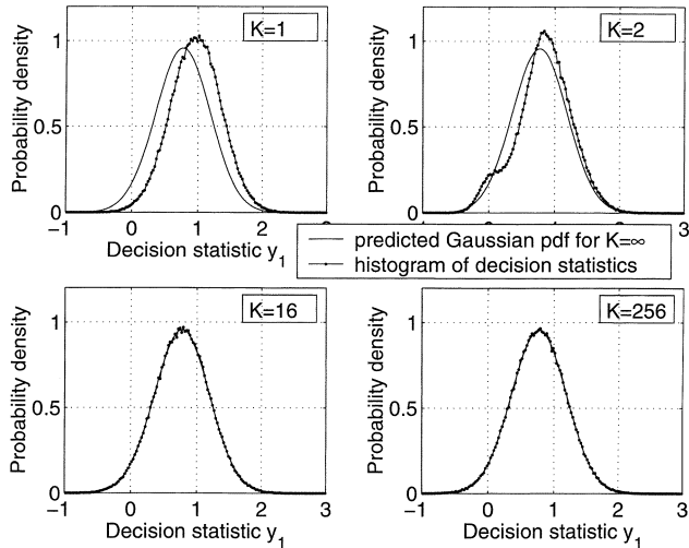
Fig. 3. Distribution of output decision statistics. The two-user, 16-user, and 256-user cases are shown as well as the single-user case ( K = 1 ). They are compared with the asymptotic Gaussian distribution.
