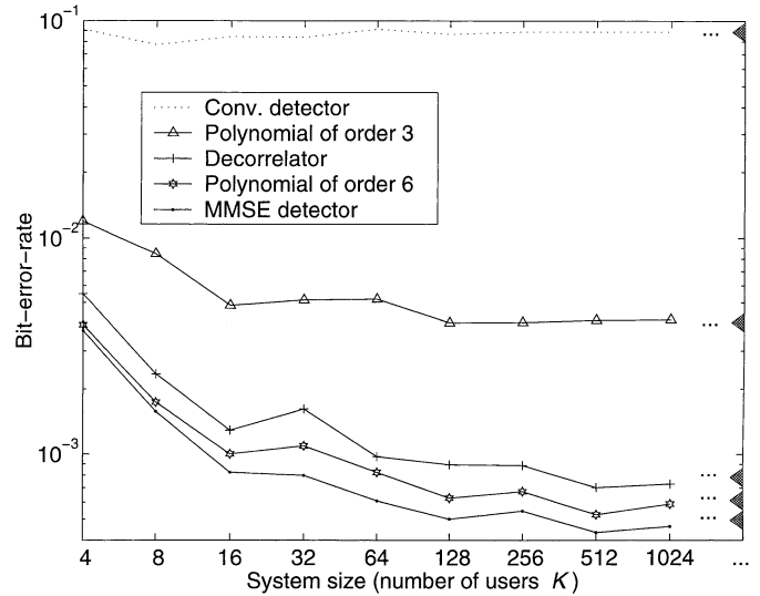
Fig. 5. BER versus the number of users (short sequences). The asymptotic estimates are marked by solid triangles on the right border of the plot.
