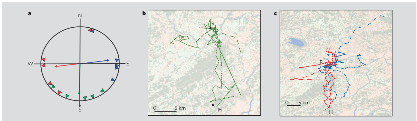
Figure 1 | Headings and tracks of homing bats. a , Heading directions at 5 km after release 20 km north of the home roost (to south; black arrow). Arrowheads, directions for individual bats; arrows, mean direction for the group. Red, anticlockwise (ACW) rotation of magnetic field by 90° with respect to north; blue, clockwise (CW) rotation of magnetic field by 90°; green, controls (no rotation of magnetic field). Orientation was significantly southerly in controls (V test, 180^\circ , U = 2.862 , P = 0.0072 ); westerly in ACW bats (V test, 270^\circ , U = 1.973 , P = 0.023 ); and easterly in CW bats (V test, 90^\circ , U = 2.66 , P = 0.002 ). Headings differed significantly between the three groups (Watson–Williams 3-sample test: F = 16.808 , P = 0.00033 ; pairwise: CW vs control, F = 23.774 , P = 0.001 ; ACW vs control, F = 6.733 , P = 0.032 ; ACW vs CW, F = 23.503 , P = 0.001 ). b , c , Control ( b ) and experimental tracks ( c ) of bats, with different dotted and dashed lines for individual bats ( n = 5 in each group). Colours indicate direction of rotation of magnetic field, as in a . R, release site; H, home.
