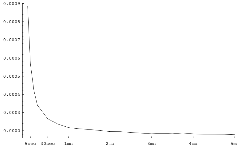
Fig. 1. This figure shows the RV estimator [Y, Y]_T^{(all)} plotted against the sampling interval \Delta = T/n . The RV estimator in the figure is computed for an average of the 30 Dow Jones Industrial Average stocks, averaged again over the last ten trading days in April 2004; the objective of the double averaging is to reduce the variability of the estimator in order to display its bias. Since \Delta = T/n , the plot illustrates the divergence of RV as n \rightarrow \infty predicted by our theory: RV has bias 2nE[\varepsilon^2] .
