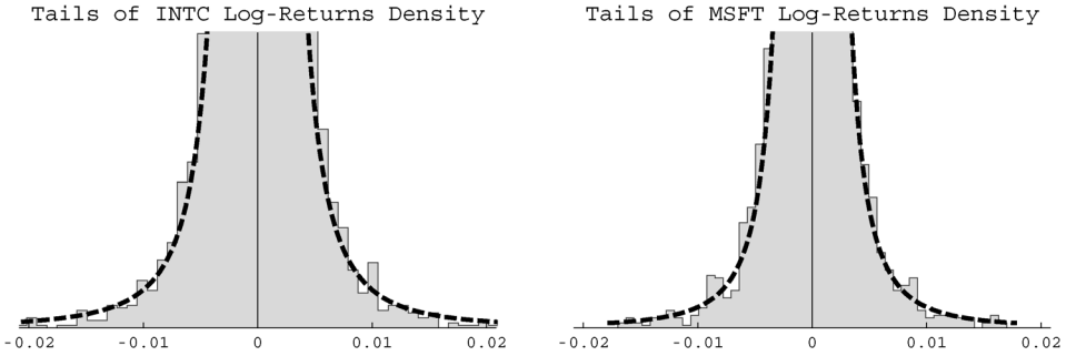
FIG. 5. Tails of the marginal density of INTC and MSFT log-returns, all trading days in 2006 sampled at 5 second intervals. The dashed curve is the leading part of the Lévy measure, that is F'_1(dx) given in (8), with jump activity index \beta , estimated for each stock by \hat{\beta}_n .
