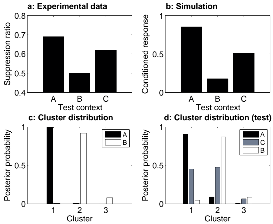
Figure 2: Renewal
