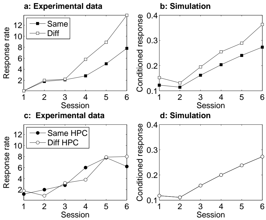
Figure 3: Latent inhibition
