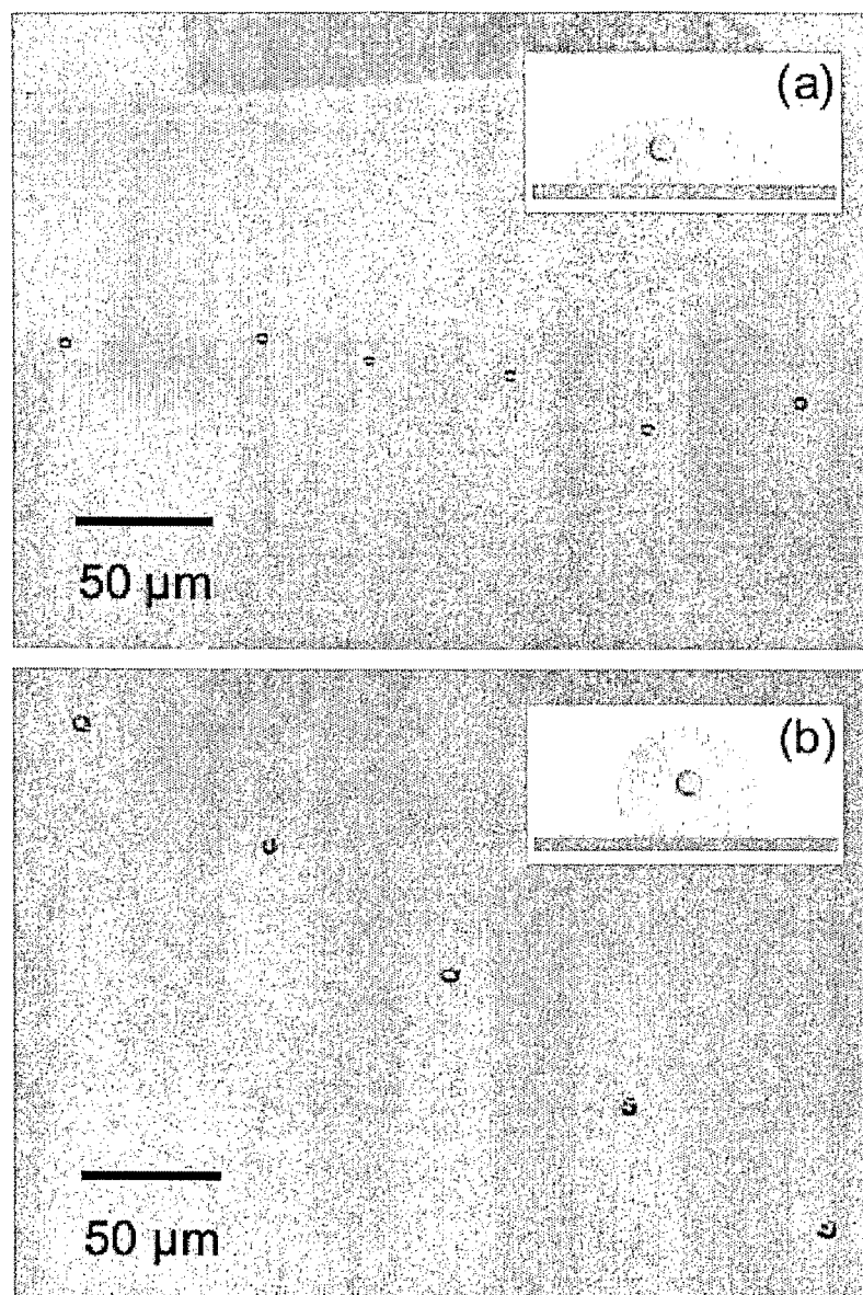
Figure 25: Improved positioning accuracy on a less wettable surface.
