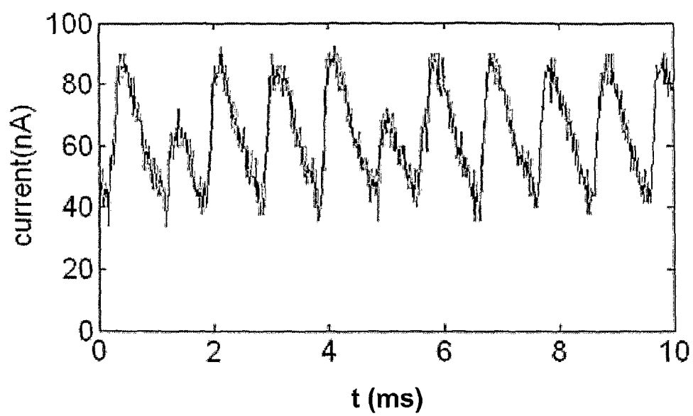
Figure 22: Current measurement in the EHD circuit.
