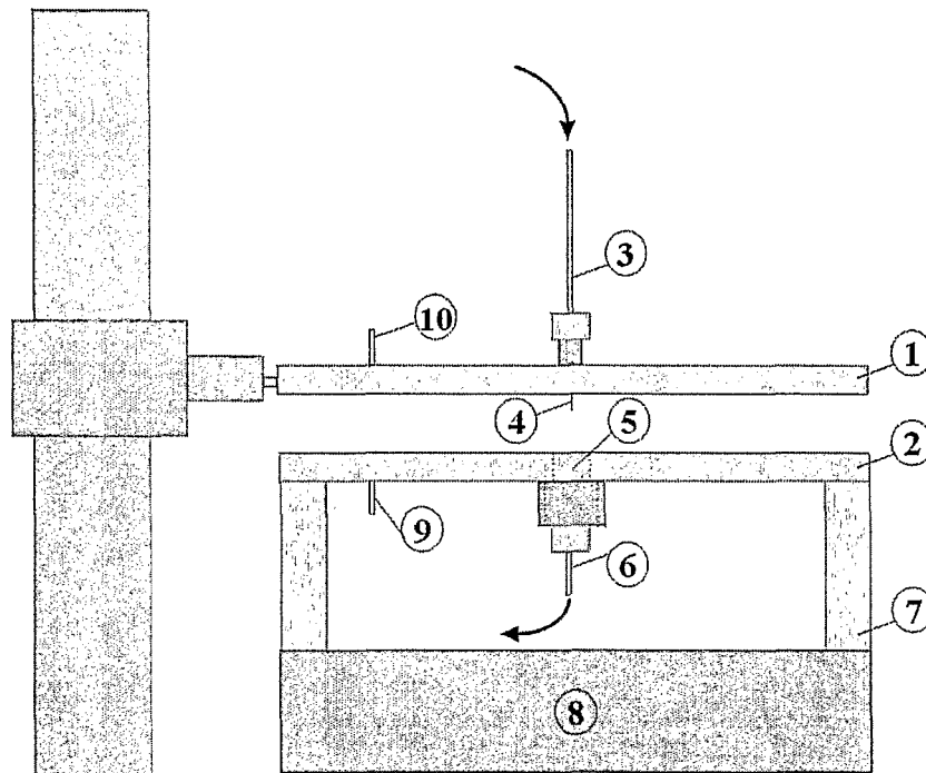
Figure 1: Experimental setup for stability experiments
