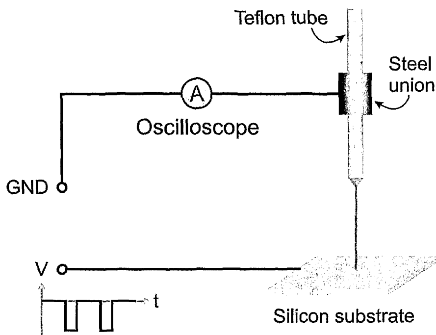
Figure 18: Experimental setup for pulsed EHD drop generation.
