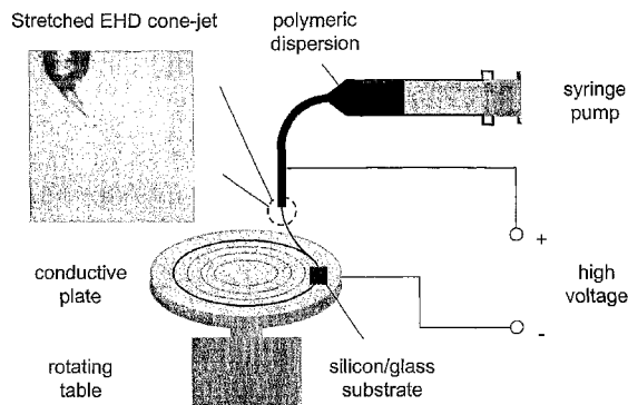
Setup for electrohydrodynamic printing of polymer fiber.
