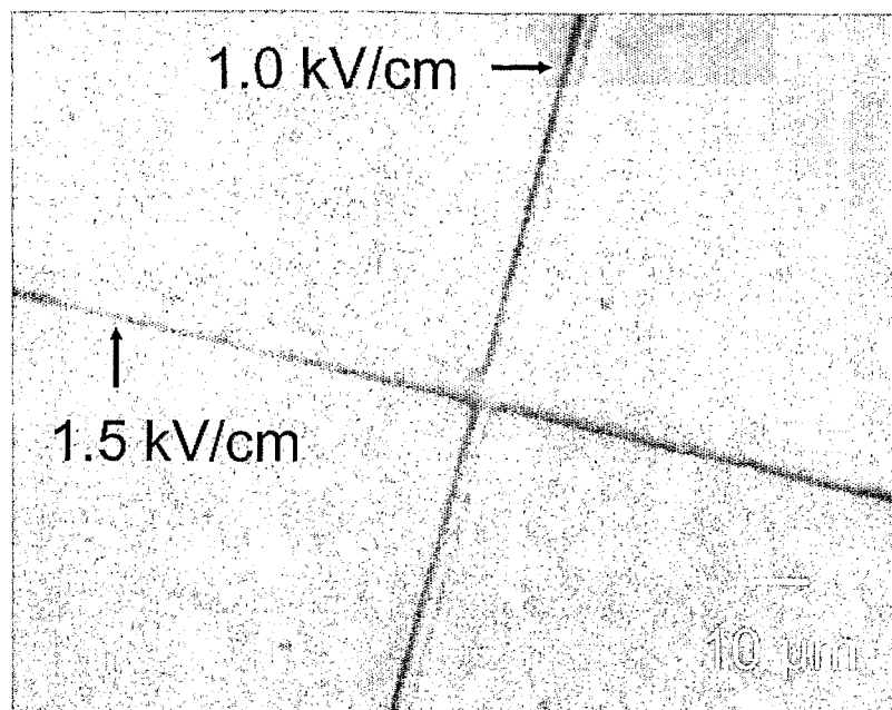
Figure 8. Fiber diameter controlled by electric field.
