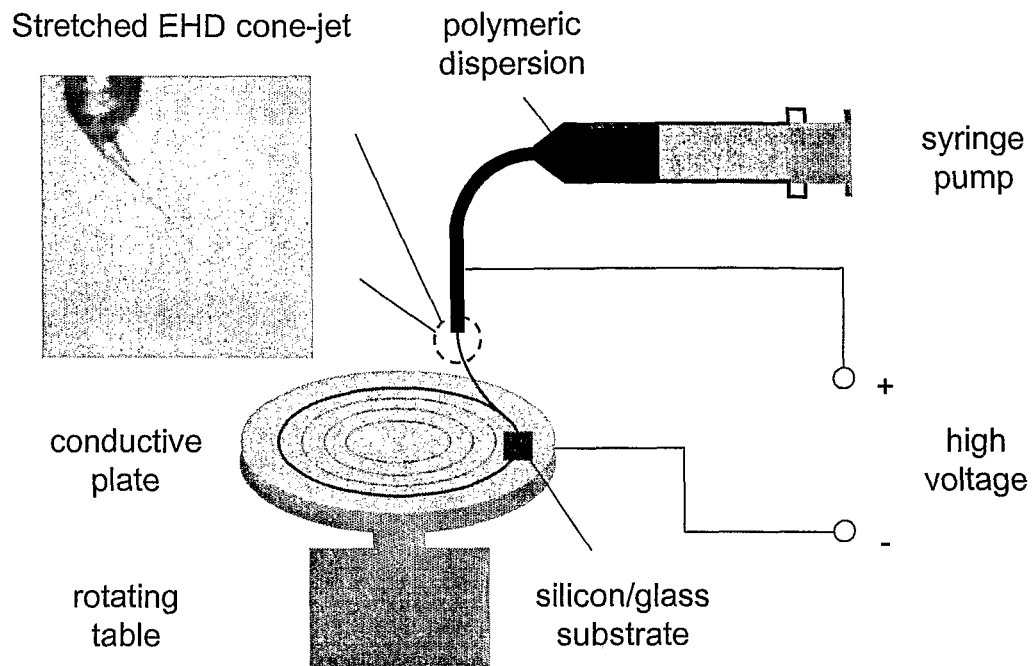
Figure 5. Setup for electrohydrodynamic printing of polymer fiber.
