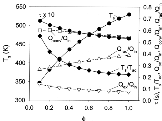
FIG. 4. Predicted reactor temperature, residence time, energy loss distributions, and thermal efficiency for a total volumetric flow rate of 80 cm 3 /min.
