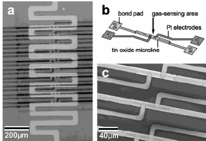
Fig. 4. Gas sensor fabricated by Heule and Gauckler [42] using micromolding in capillaries. (a) Top view as viewed through an optical microscope in which the dark horizontal lines are the patterned tin oxide features. (b) Schematic of the device. (c) SEM image of the device showing the platinum contact lines contacting the tin oxide features.
