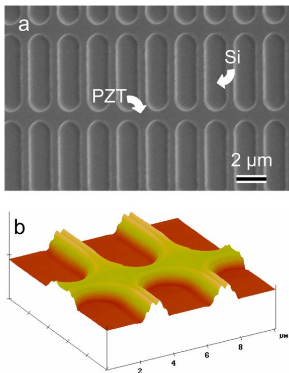
Fig. 3. (a) SEM image of a grid pattern of PZT lines patterned from 1\text{ }\mu\text{m} wide channels. (b) AFM topography scan of 2\text{ }\mu\text{m} wide PZT lines that shows the “double-peak” topographical distortion that forms during drying and sintering.
