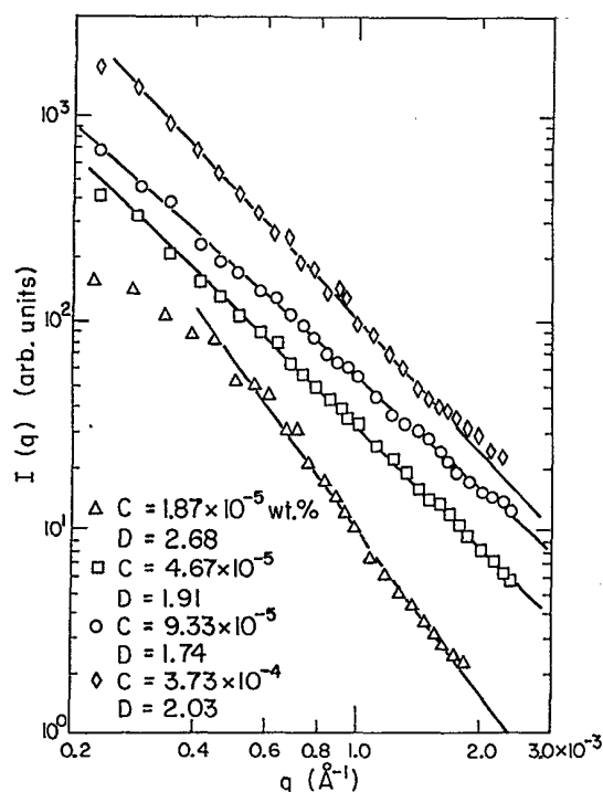
FIG. 2. Static light-scattering intensity of the aggregated samples corresponding to Fig. 1(b) D=2.68 ( \Delta ), Fig. 1(c) D=1.91 ( \square ), Fig. 1(d) D=1.74 ( \circ ), and Fig. 1(e) D=2.03 ( \diamond ), where D is the fractal dimension of the aggregates.
