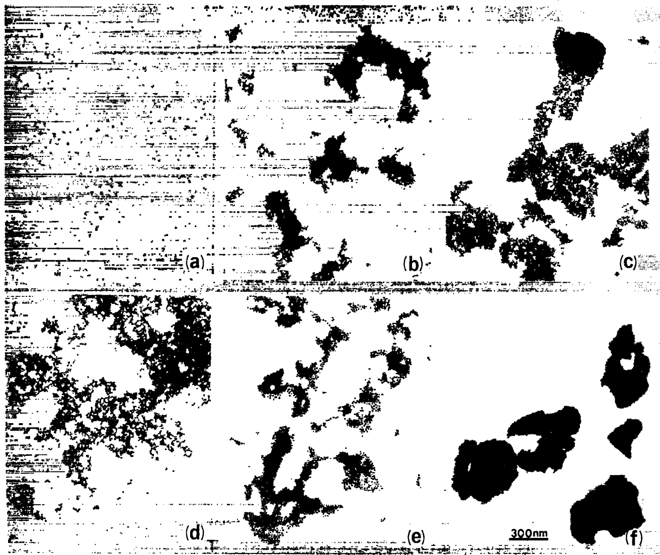
FIG. 1. TEM micrographs of gold particles at various surfactant concentrations c : (a) c = 0 , (b) 1.87 \times 10^{-5} , (c) 4.67 \times 10^{-5} , (d) 9.33 \times 10^{-5} , (e) 3.73 \times 10^{-4} , and (f) 5.61 \times 10^{-4} wt. %.
