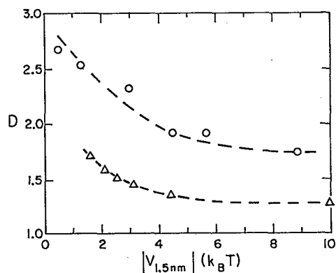
FIG. 6. D vs |V_{1.5 \text{ nm}}| for the aggregated samples ( \circ ), where D is the fractal dimension and |V_{1.5 \text{ nm}}| is the net interparticle attraction energy at s = 1.5 nm. Also plotted is D vs |E| from the computer simulations of Ref. 12 ( \triangle ), where |E| is the nearest-neighbor attraction energy in Ref. 12. Both |V_{1.5 \text{ nm}}| and |E| are in units of k_B T .
