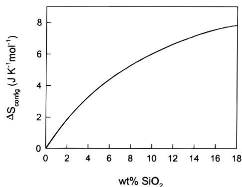
Figure 4. Calculated (using eqs 10–12) entropies of formation of the aluminosilicate solid solutions relative to a mechanical mixture of \alpha - \text{Al}_2\text{O}_3 and quartz as a function of \text{SiO}_2 content.
