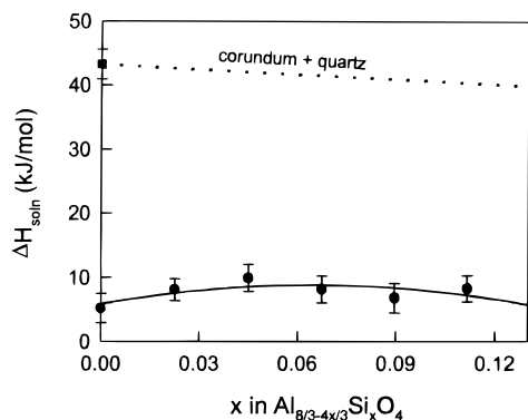
Figure 2. Enthalpies of solution of the aluminosilicate solid solutions in 2\text{PbO} \cdot \text{B}_2\text{O}_3 at 1043 K as a function of \text{SiO}_2 content. Dotted line represents the values expected from a mechanical mixture of coarse \alpha\text{-Al}_2\text{O}_3 and quartz.
