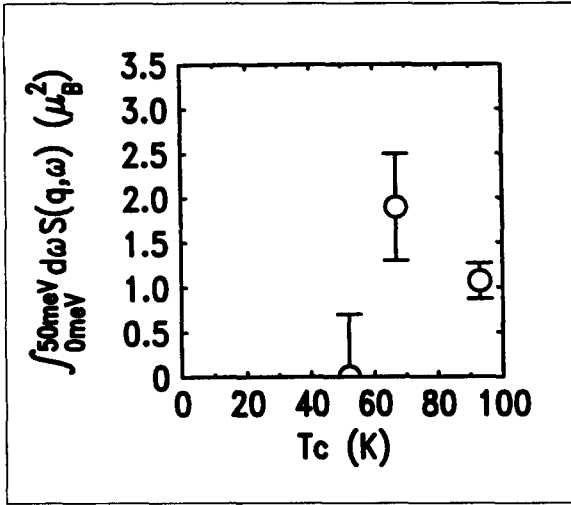
Figure 5. Energy integral of S(q, \omega) at q = (\pi, \pi) and 0 \leq \hbar\omega \leq 50 meV, for different doping levels.
