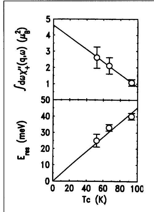
Figure 4. T_c -dependence of the enhanced part of the dynamical susceptibility, \int d\omega \chi''_+(\mathbf{q}, \omega) , and the resonance energy E_{\text{res}} .
