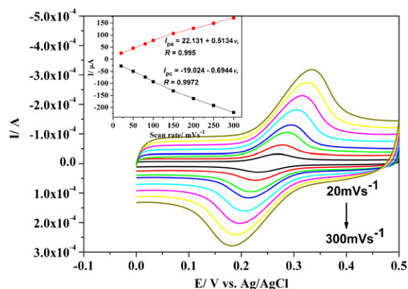
Fig. 3. CVs acquired on graphene/GCE with 20 μM paracetamol in the buffer of NH 3 ·H 2 O–NH 4 Cl (0.1 M pH 9.3) at different scan rates from 20 to 300 mV s -1 . Inset is the plot of the peak current of paracetamol versus scan rate.
