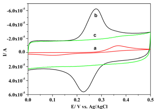
Fig. 2. CVs recorded at a bare GCE (a) with 100 μM paracetamol; graphene/GCE with (b) 20 μM paracetamol and without paracetamol (c) in the buffer of 0.1 M NH 3 ·H 2 O–NH 4 Cl, pH 9.3, scan rate: 50 mV s -1 .
