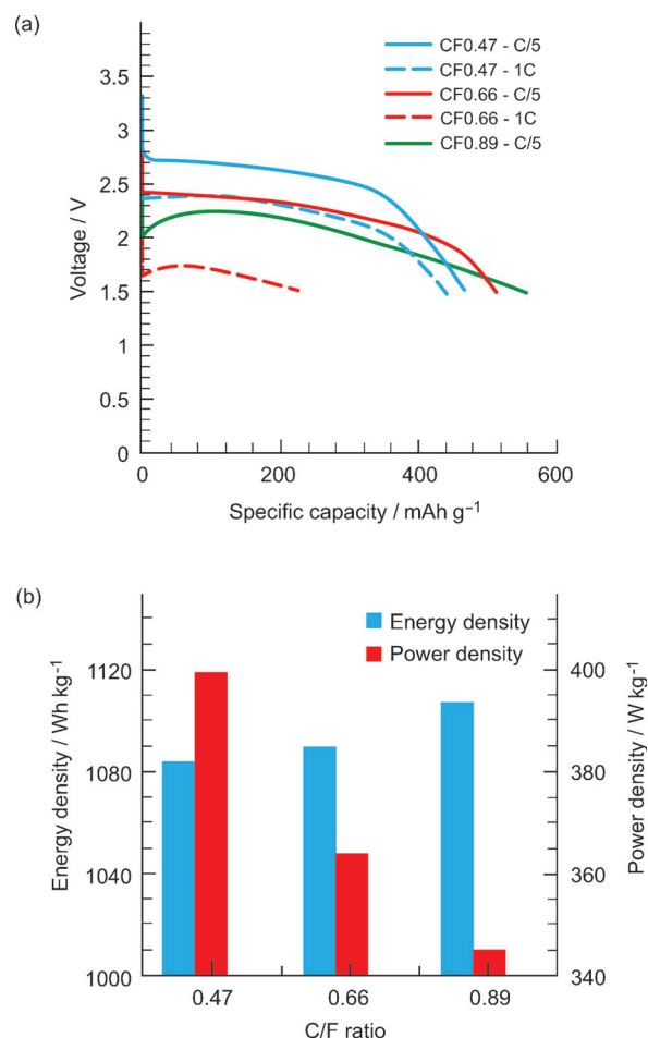
Figure 3. (a) Rate performance of fluorinated graphene materials (1C current density for \text{CF}_{0.47} —602 \text{mA g}^{-1} ; \text{CF}_{0.66} —721 \text{mA g}^{-1} ; \text{CF}_{0.89} —825 \text{mA g}^{-1} ). (b) Comparison of gravimetric energy and power densities of fluorinated graphene at C/5 rate.
