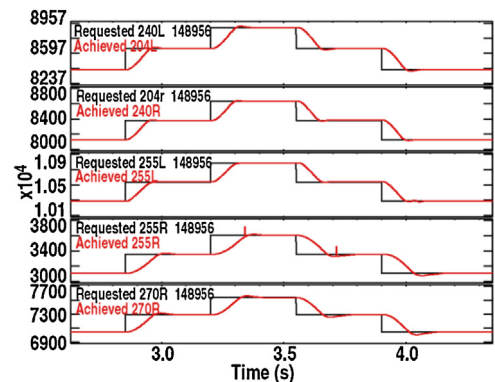
Fig. 4. Multiple step response of the mirror control.
