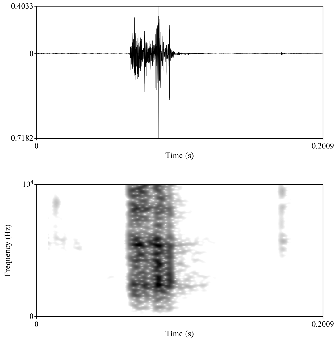
Figure 4: lateral click [l̥] (AK, elicited, careful speech)
