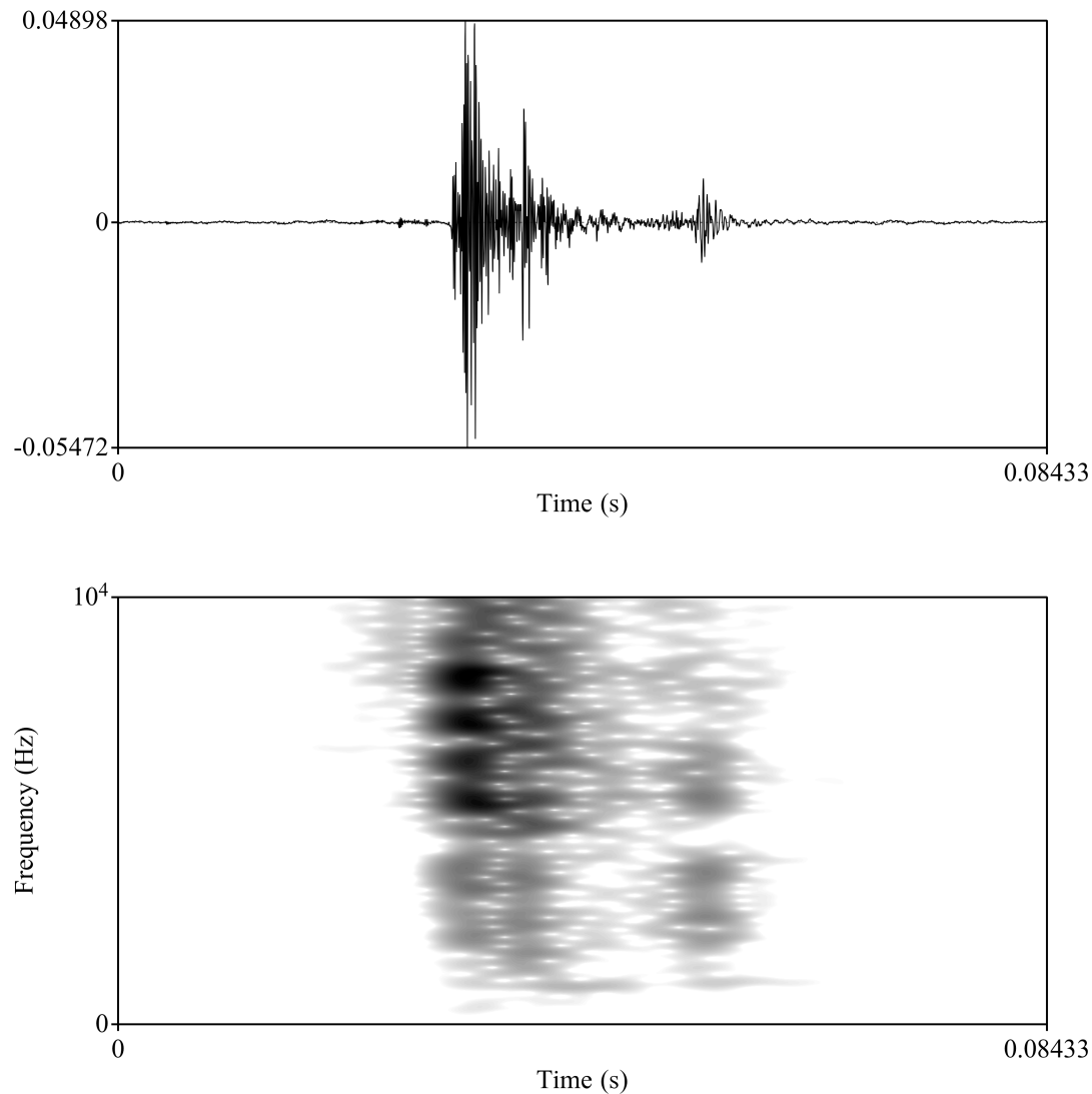
Figure 2: Dental click [ǀ] (Speaker KD, natural speech)
