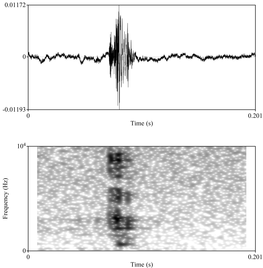
Figure 6: Velar click, (speaker AK, elicited, careful speech)
