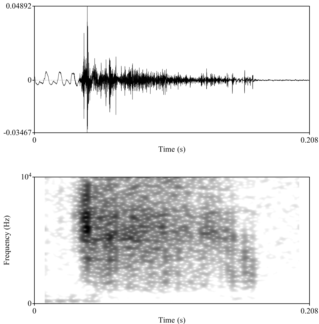
Figure 7: “Tchip” (speaker KD, natural speech)
