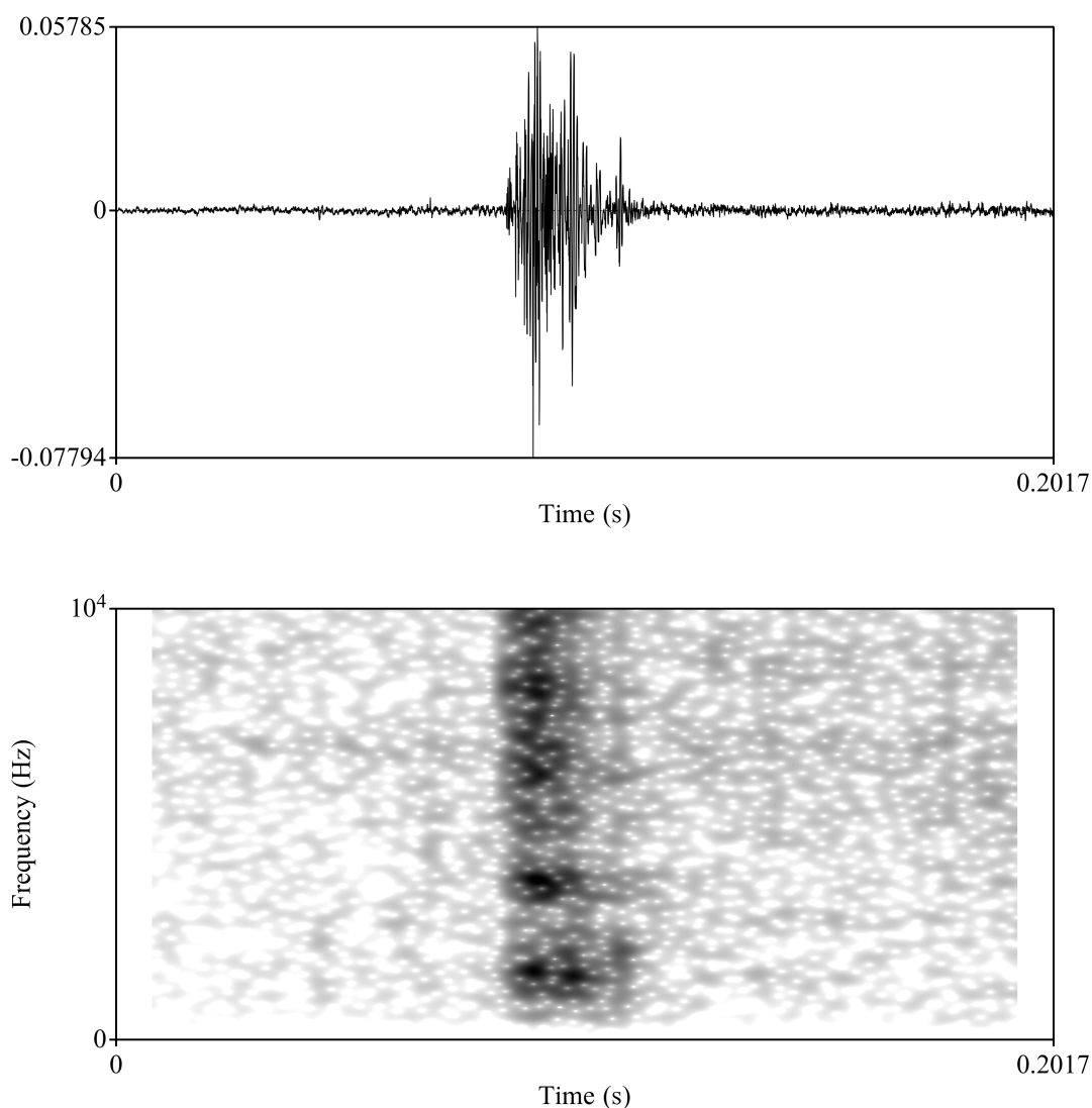
Figure 3: lateral click [ɭ] (speaker ID, natural speech, Zoom H4n built-in microphone)
