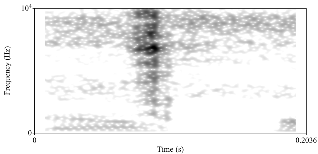
Figure 1: Dental click [ɿ] (Speaker ID, natural speech, Zoom H4n built-in microphone)
