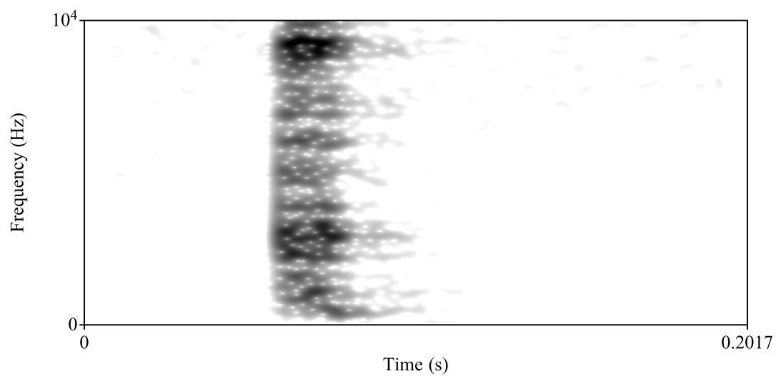
Figure 5: Velar click (speaker KD, elicited, careful speech)
