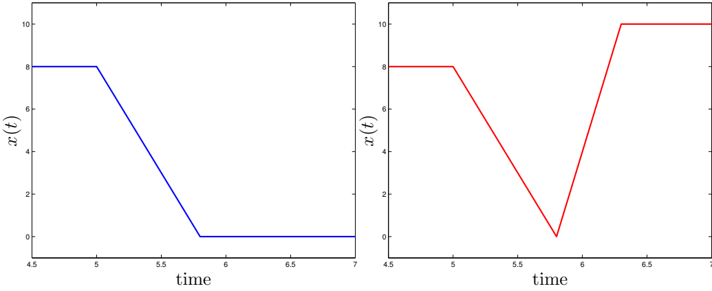
Figure 1: Holdings of Distressed Trader (Panel A) and of Single Predator (Panel B). Starting with an initial holding of x^i(t_0) = 8 , both traders sell at maximum intensity of A/2 = 10 from t_0 = 5 until t_0 + \frac{x(t_0)}{A/2} = 5.8 . By then, the distressed trader has completed his liquidation and subsequently the predator buys back shares.
