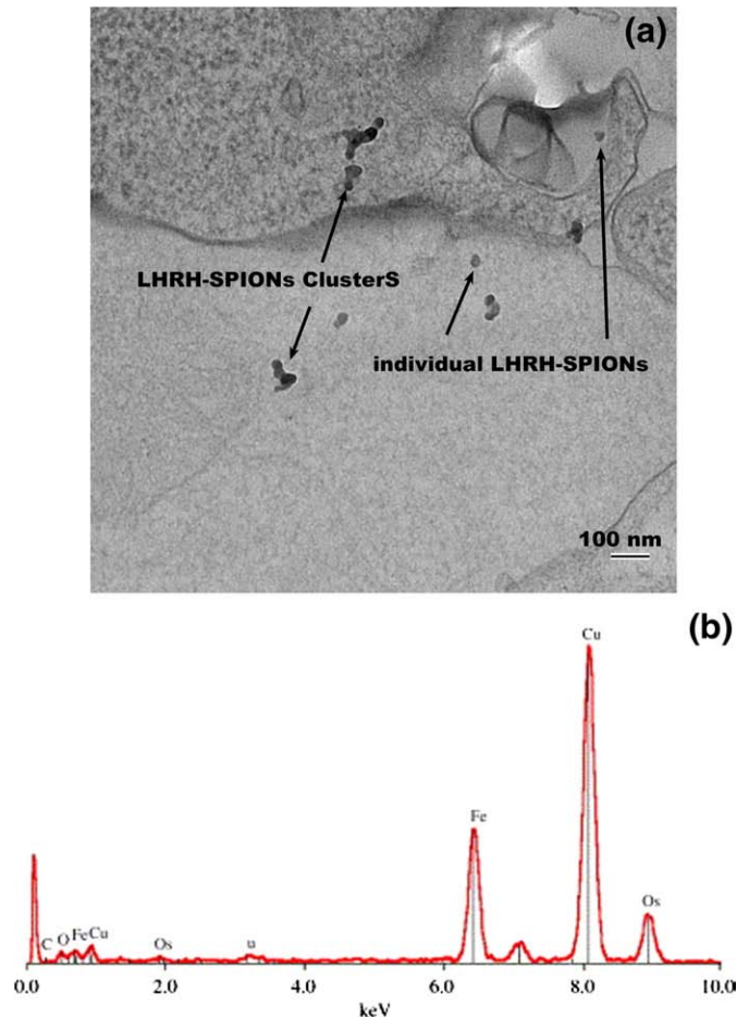
Fig. 11. (a) TEM micrographs of breast cancer cells from a female mouse injected with LHRH-SPIONs. Both individual particles and particle clusters distributed in the cell. (b). An XEDS spectrum collected from SPIONs distributed in tumor cells.
