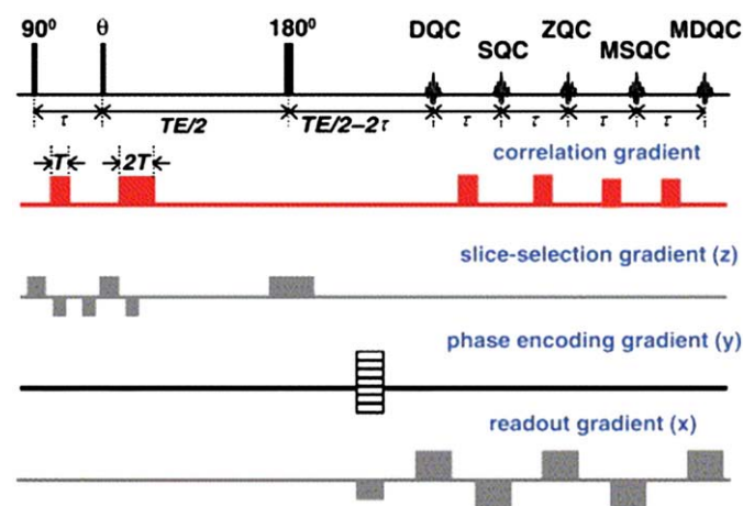
Fig. 1. Multi-CRAZED sequence to acquire multiple echoes. The multi-CRAZED sequence takes advantage of the difference in echo timing to acquire multiple echoes at full intensity. The + SQC (+1 or single-quantum coherence) and MSQC (–1 or single-quantum coherence) images have primarily conventional contrast; the DQC (+2-quantum), ZQC (0-quantum), and MDQC (–2-quantum) coherences have contrast from subvoxel variations in magnetization density or resonance frequency. Additional gradient pulses permit image acquisition in the standard way (single-line acquisition shown here) (adapted from Ref. [20]).
