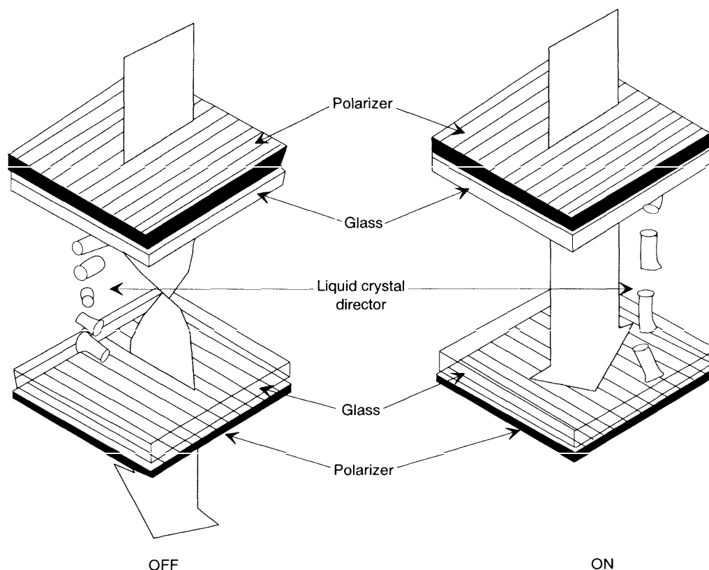
FIGURE A-1: Twisted Nematic Liquid Crystal Cell
