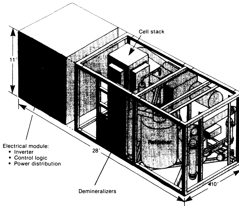
Figure 40-21.—Design for a 200 kWe Fuel Cell Module
