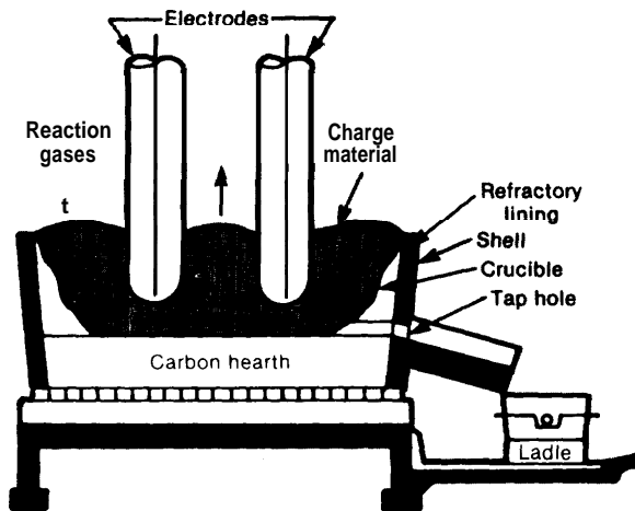
Figure 5-2.—Submerged Arc Furnace
