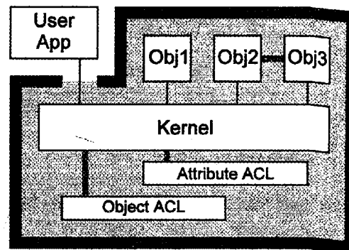
Figure 4: cryptlib architecture
