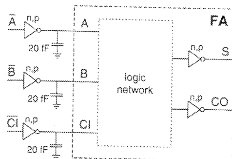
Fig. 2. Circuit arrangement for the simulation of full-adders.
