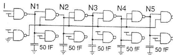
Fig. 3. Circuit arrangement for the simulation of logic gates.
