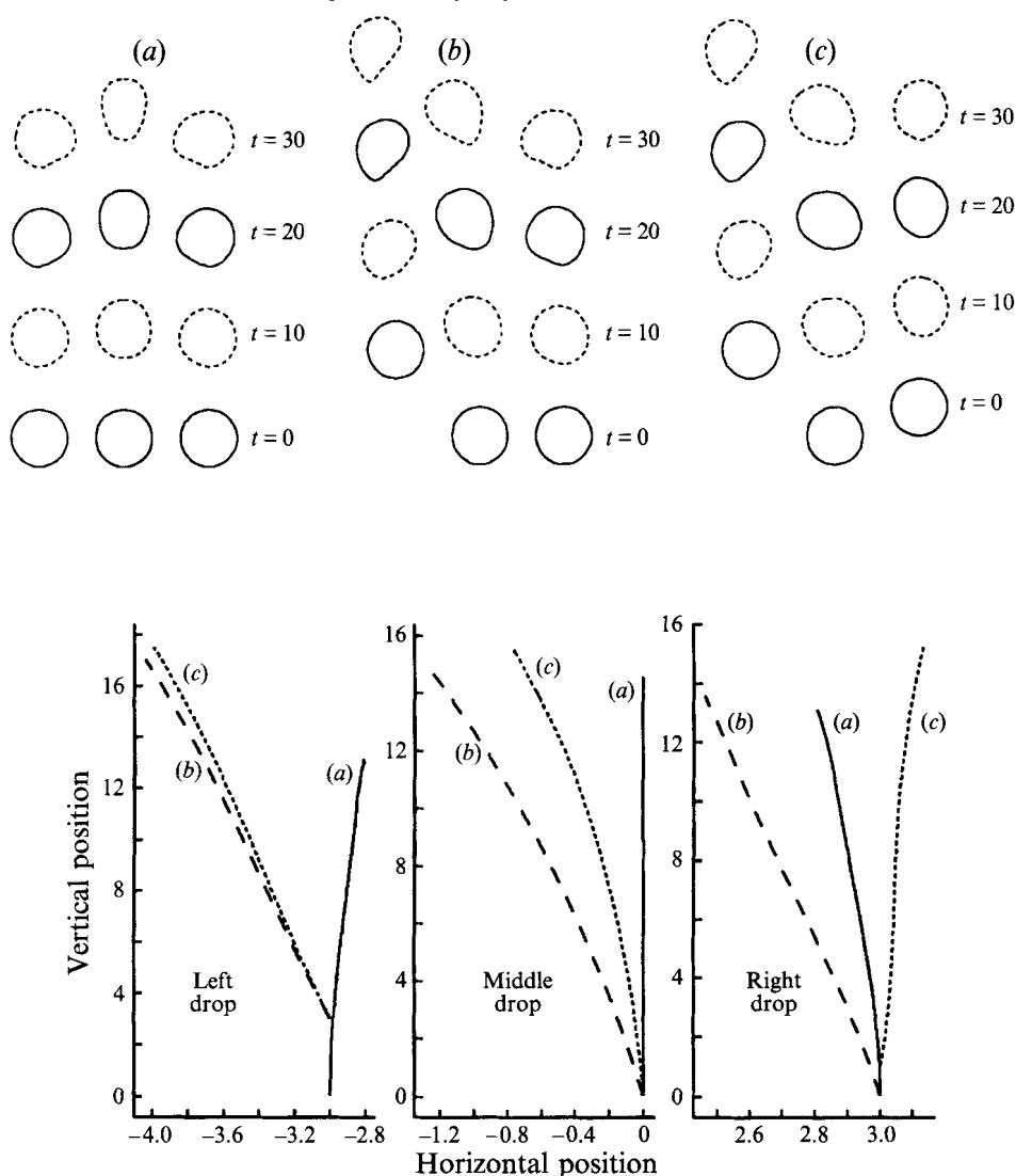
FIGURE 7. Shapes of three-dimensional drops, for three equal-size drops with different initial vertical offsets but identical horizontal offsets; \mathcal{B} = 10 , \lambda = 1 . Cross-sections of drop shapes are shown.
