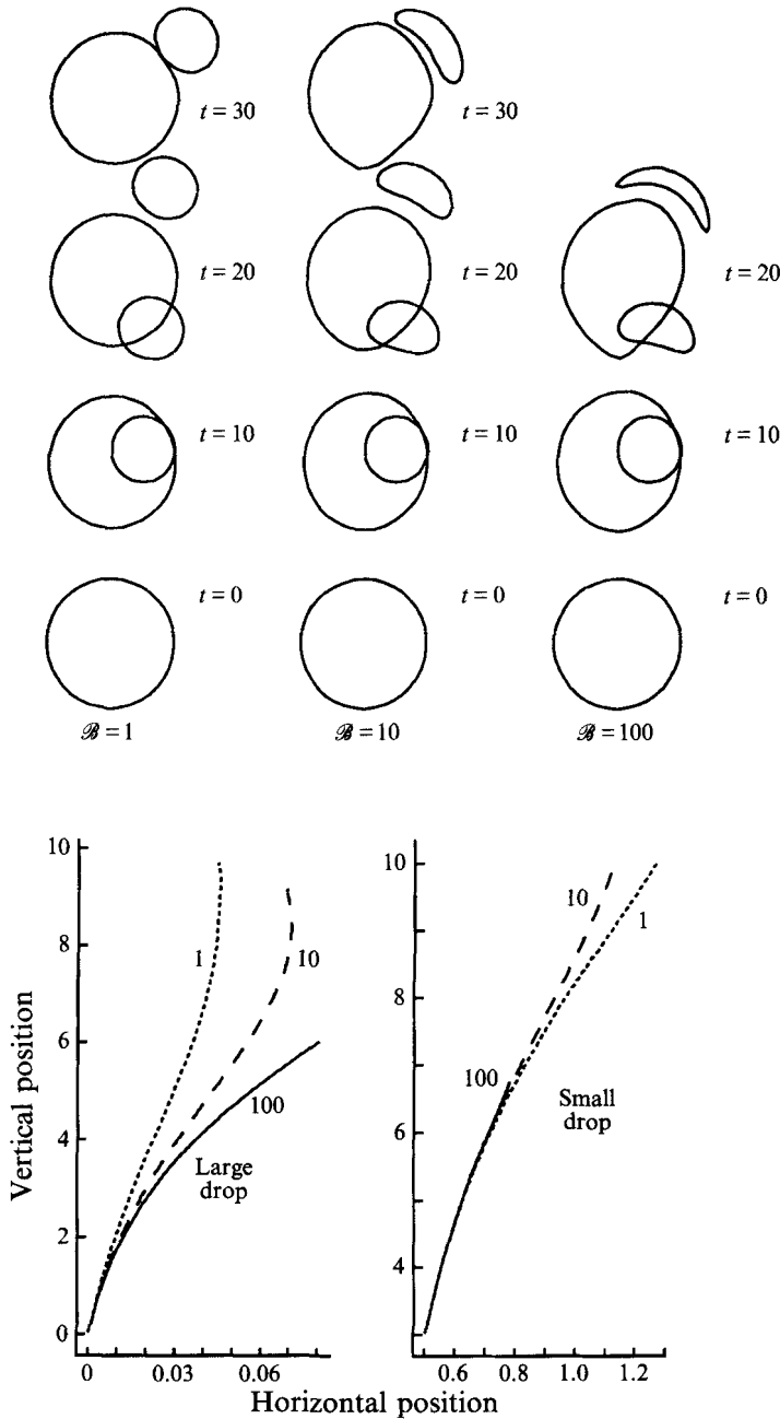
FIGURE 4. The effect of interfacial tension (Bond number) on the alignment of three-dimensional offset drops for Bond numbers of the larger trailing drop B = 1, 10 and 100 ; \lambda = 1 , a_2/a_1 = 0.5 . Cross-sections of three-dimensional shapes are shown. Drop trajectories are shown in the lower figure. Time is normalized by an advective timescale, \mu/\Delta\rho g a_1 , where a_1 is the radius of the larger drop.
