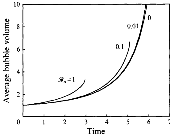
FIGURE 17. Average normalized bubble volume as a function of time in isotropic homogeneous suspension. Time is normalized by \mu/\Delta\rho g a_o \phi_o . Results are presented for \mathcal{B}_o = 0, 0.01, 0.1 and 1 . The Bond number is based on the average initial bubble radius a_o .
