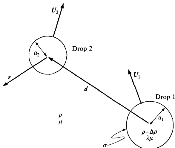
FIGURE 3. Two-drop geometry.
