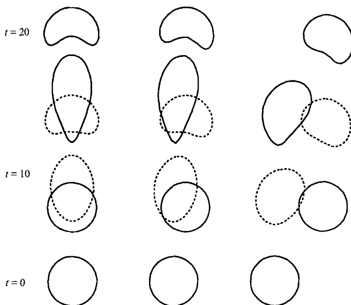
FIGURE 11. Shapes of two three-dimensional drops, for equal-size drops with different initial horizontal offsets; B = 10 , \lambda = 1 . Cross-sections of drop shapes are shown.
