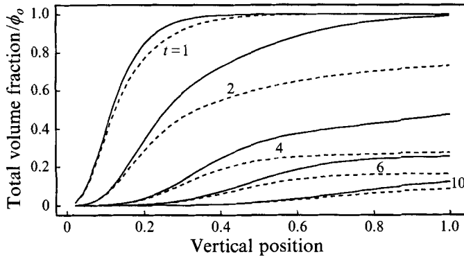
FIGURE 19. Total volume fraction of bubbles, normalized by the initial volume fraction \phi_o , as a function of tank height (0=bottom, 1=top), at dimensionless times t = 1, 2, 4, 6 and 10 . Results are presented for \mathcal{B}_o = 1 (dashed lines) and \mathcal{B}_o = 0 (solid lines). Time is normalized by \mu/\Delta\rho g a_o \phi_o . The height of the tank is normalized by 50a_o/\phi_o . The Bond number is based on the average initial bubble radius a_o .
