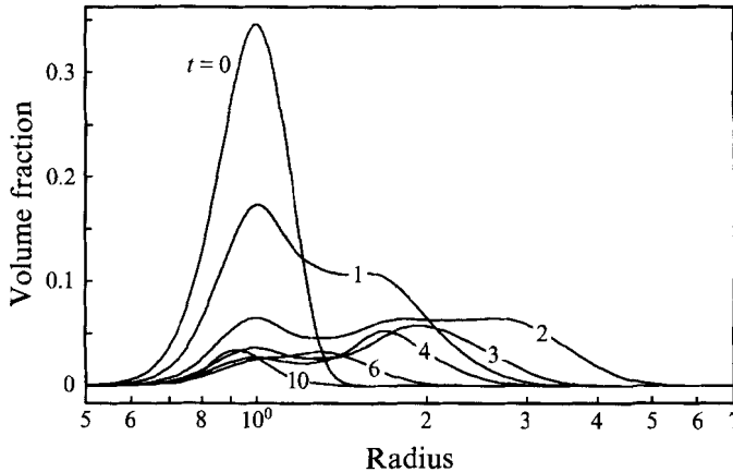
FIGURE 20. The size distribution of bubbles at the top of the tank, at dimensionless times t = 0, 1, 2, 3, 4, 6 and 10 ; \mathcal{B}_o = 1 . Time is normalized by \mu/\Delta\rho g a_o \phi_o . The height of the tank is 50a_o/\phi_o . The Bond number is based on the average initial bubble radius a_o .
