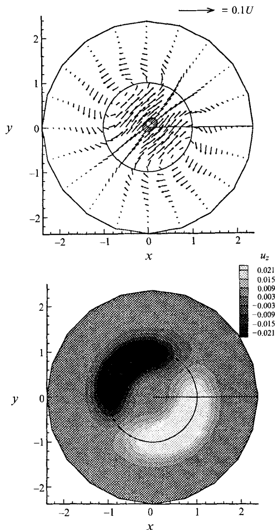
FIGURE 8. Plan view through z/\mathcal{F} = 0.01 showing the far field for \mathcal{F} = 500 . The unit disk is centred at the origin and translates along the x -axis from left to right. The top figure shows the velocity field in the plane; the bottom figure is a contour plot of the axial velocity field. Two counter-rotating eddies centred over the edge of the disk create a net flow directed at an angle \theta = -45^\circ and 135^\circ from the translation direction. The eddies are regions of the largest axial flow observed outside the Ekman layer (see figures 9 and 10).
