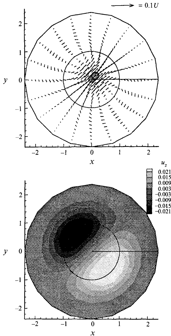
FIGURE 9. Plan view showing the far field at a section through z/\mathcal{F} = 0.05 for \mathcal{F} = 500 (see figure 8).
