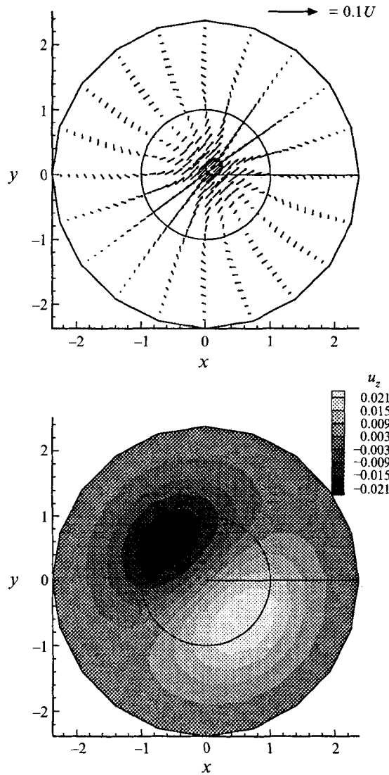
FIGURE 10. Plan view showing the far field at a section through z/\mathcal{F} = 0.075 for \mathcal{F} = 500 (see figure 8).
