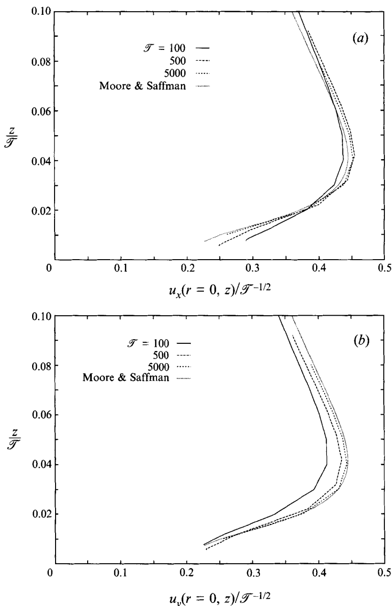
FIGURE 5. The velocity field u_x(r=0, z/\mathcal{T}) and u_y(r=0, z/\mathcal{T}) in the region outside the Ekman layer. The magnitude of the velocity is scaled by \mathcal{T}^{-1/2} ; the distance from the disk surface is scaled by \mathcal{T} . The results, which collapse to a single curve in the high Taylor number limit, are in agreement with the asymptotic results of Moore & Saffman (1969a) given by (3.11). Note that these scalings are inappropriate in the Ekman layer near z=0 .
