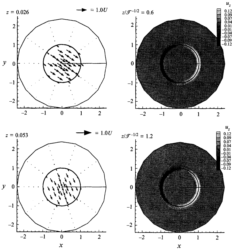
FIGURE 11. Plan view showing the Ekman layer at sections through z/\mathcal{F}^{-1/2} \approx 0.6, 1.2 for \mathcal{F} = 500 . The disk occupies the region r < 1 and moves from left to right. The figures on the left show the in-plane velocity vectors; the figures on the right show contours of the axial velocity field. The velocity vectors along the centreline spiral through nearly a full revolution as distance from the disk increases. Regions of net up-flow/down-flow occur over the leading/trailing edge. These regions rotate clockwise through 45^\circ and develop into counter-rotating eddies (see figures 12–14.)
