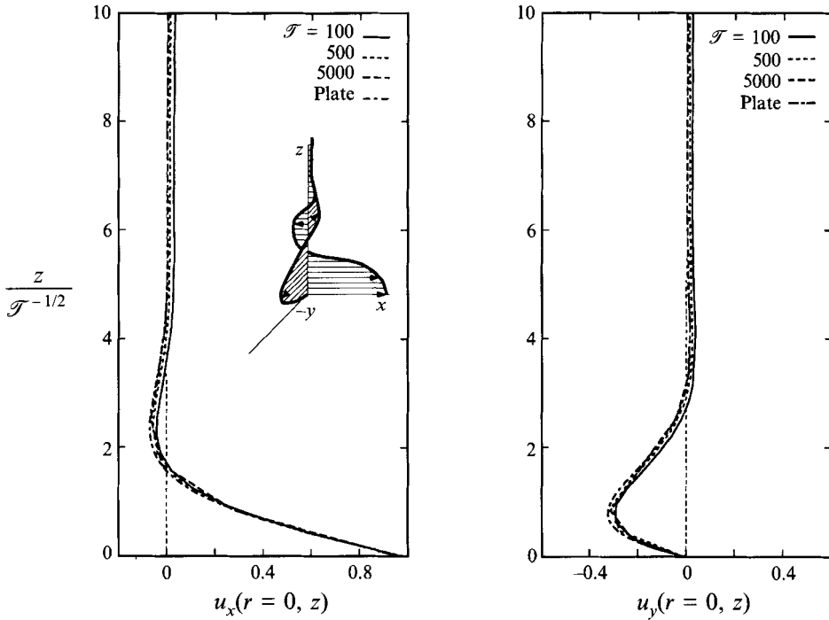
FIGURE 6. The velocity field u_x(r=0, z/\mathcal{T}^{-1/2}) and u_y(r=0, z/\mathcal{T}^{-1/2}) for positions along the centerline inside the Ekman layer adjacent to the disk surface. The distance from the disk surface is scaled by the Ekman layer thickness \mathcal{T}^{-1/2} . Also shown is the velocity field corresponding to a translating plate as given by equation (3.1).
