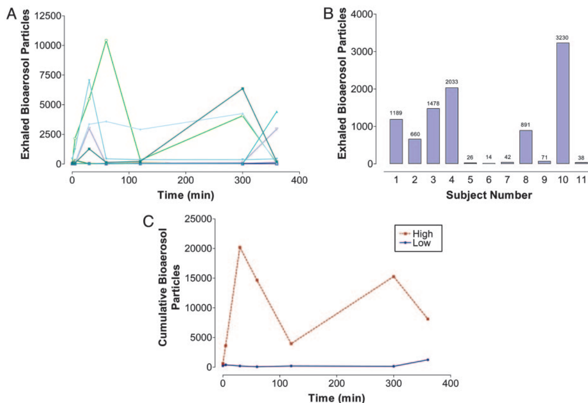
Fig. 1. Exhaled bioaerosol particles during normal breathing of 11 healthy human subjects. (A) Exhaled bioaerosol particles per liter vs. time for 11 healthy human subjects. Particles of >150 nm were counted in these measurements, after a period of 2-min expiration at each represented time point. (B) Average exhaled bioaerosol particles per liter vs. human subject over the 6-h measurement interval. The average exhaled particle per liter number was obtained by summing the measured particle numbers for every time point during the 6-h period and dividing by the number of time points. High producers are defined as those subjects who expire on average >500 particles per liter. (C) Cumulative expired particles per liter vs. time for the high- ( n = 6 subjects) and low-producer ( n = 5 subjects) groups. Cumulative expired particles were determined by summing up the expired particles per liter for all individuals of a group at each time point.
