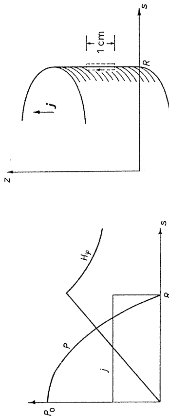
Fig. 5. The static plasma column.
